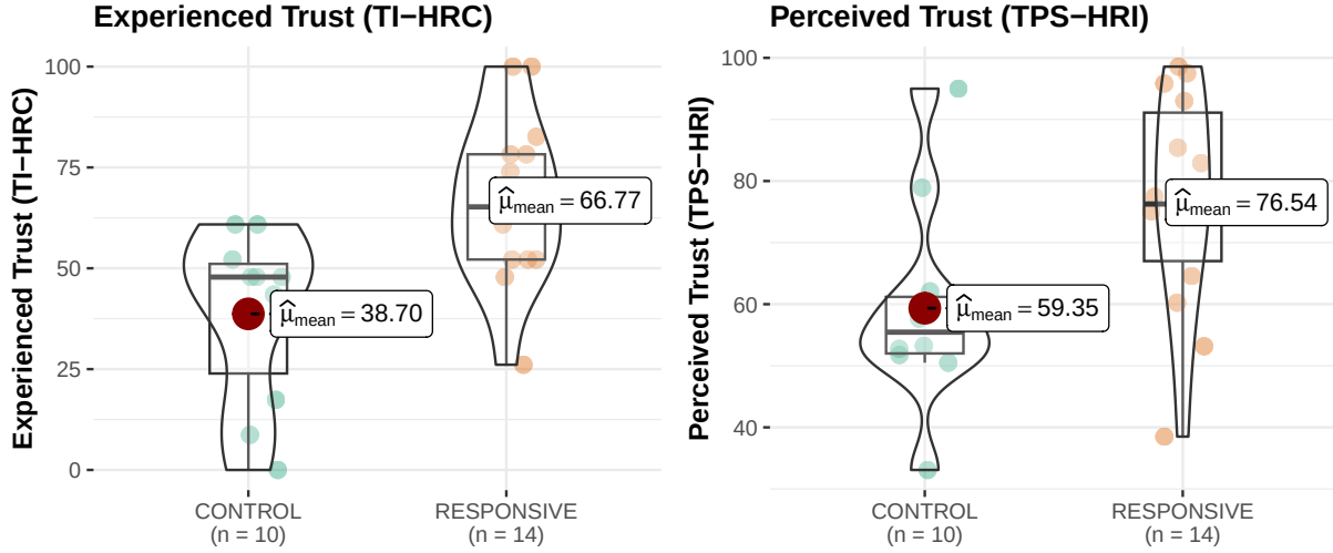
Figure 3: Distribution of Trust Perception by interaction policy. Points represent individual observations; violins depict score distributions. Red points indicate group means with 95% confidence intervals. Statistical comparisons are reported in the Results section.
