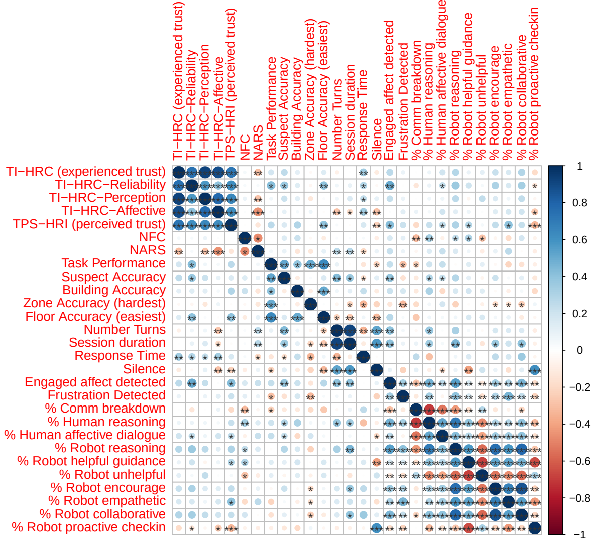
Figure 6: Correlation Matrix of Key Study Variables
