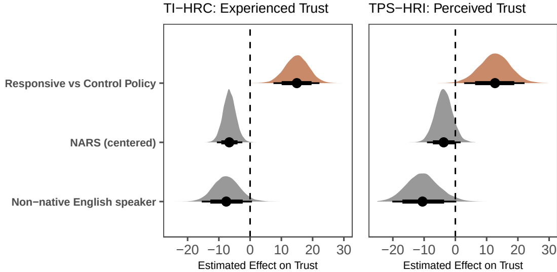
Figure 5: Posterior distributions of fixed effects from the final Bayesian mixed-effects models (eligible sample: n=24 ) predicting post-interaction trust. Fixed effects include Responsive vs Control policy, Negative Attitudes Towards Robots (NARS) and Non-native English speaker versus English native speaker. Half-eye densities show posterior distributions; points indicate posterior medians; thick and thin intervals denote 80% and 95% credible intervals, respectively. The dashed vertical line marks a null effect, and positive values indicate higher trust scores on the respective scale (points on a 0-100 scale).
