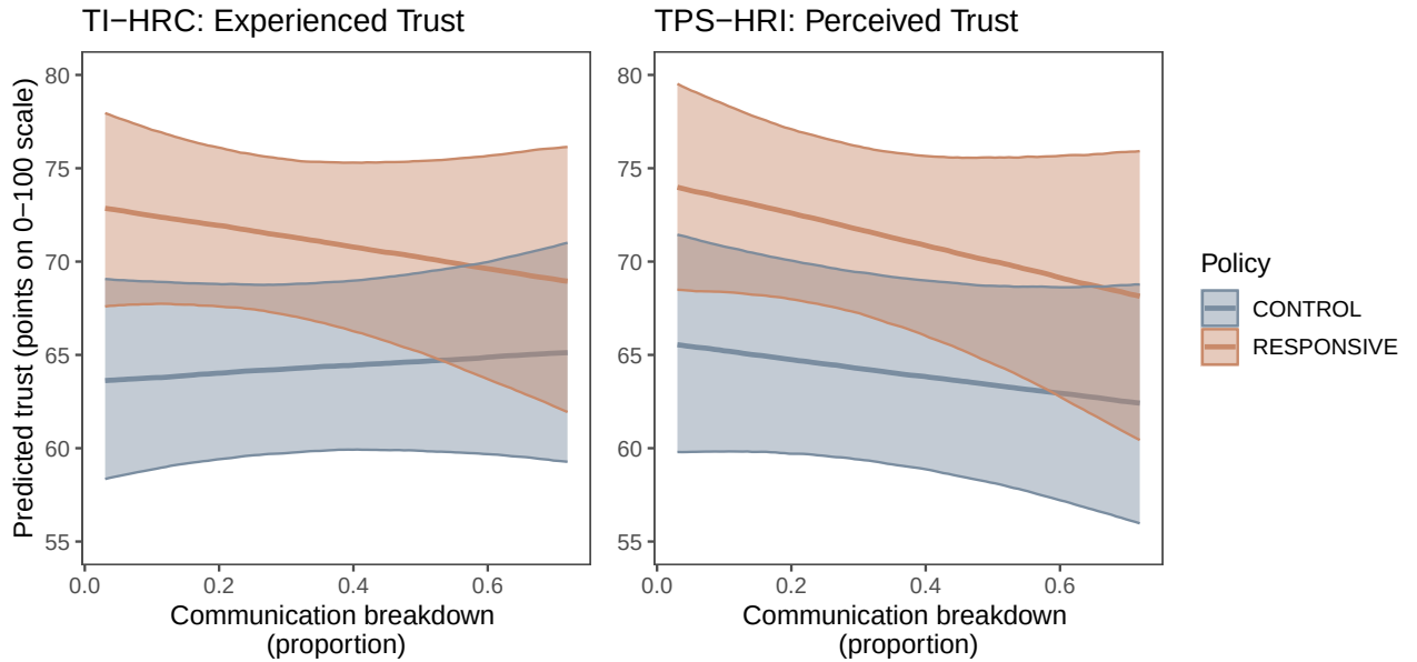
Figure 6: Predicted trust scores as a function of communication breakdown, stratified by interaction policy. Panels show experienced trust (left) and perceived trust (right). Lines represent posterior medians and shaded bands indicate 80% credible intervals. Communication breakdown is defined as the proportion of interaction turns flagged as breakdowns; predictions are shown at mean baseline negative attitudes toward robots.
