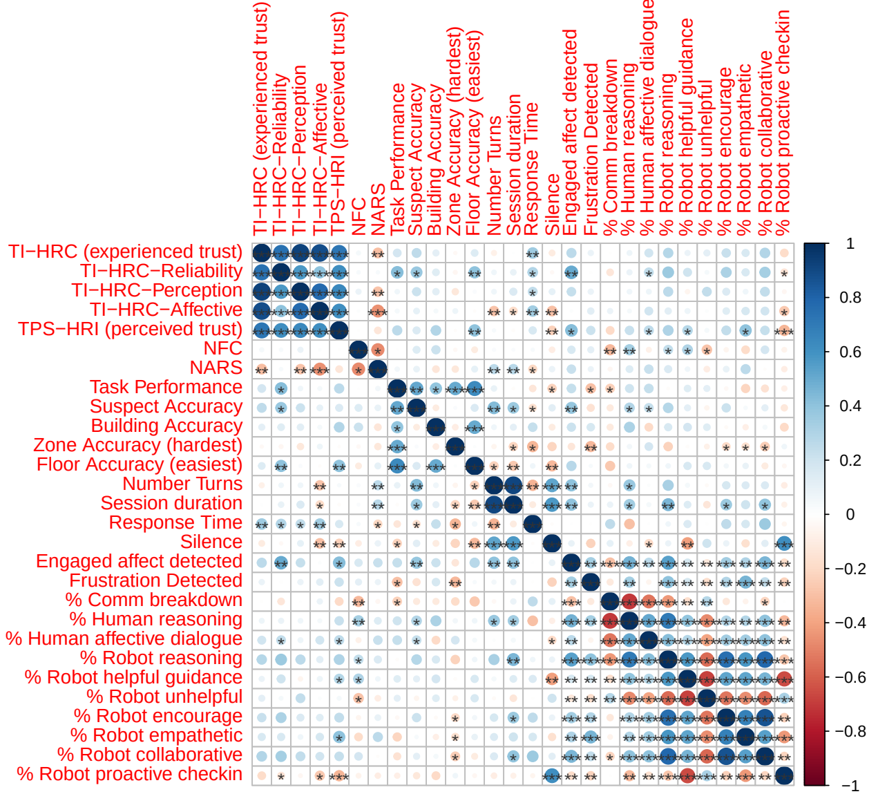
Figure 7: Correlation Matrix of Key Study Variables
