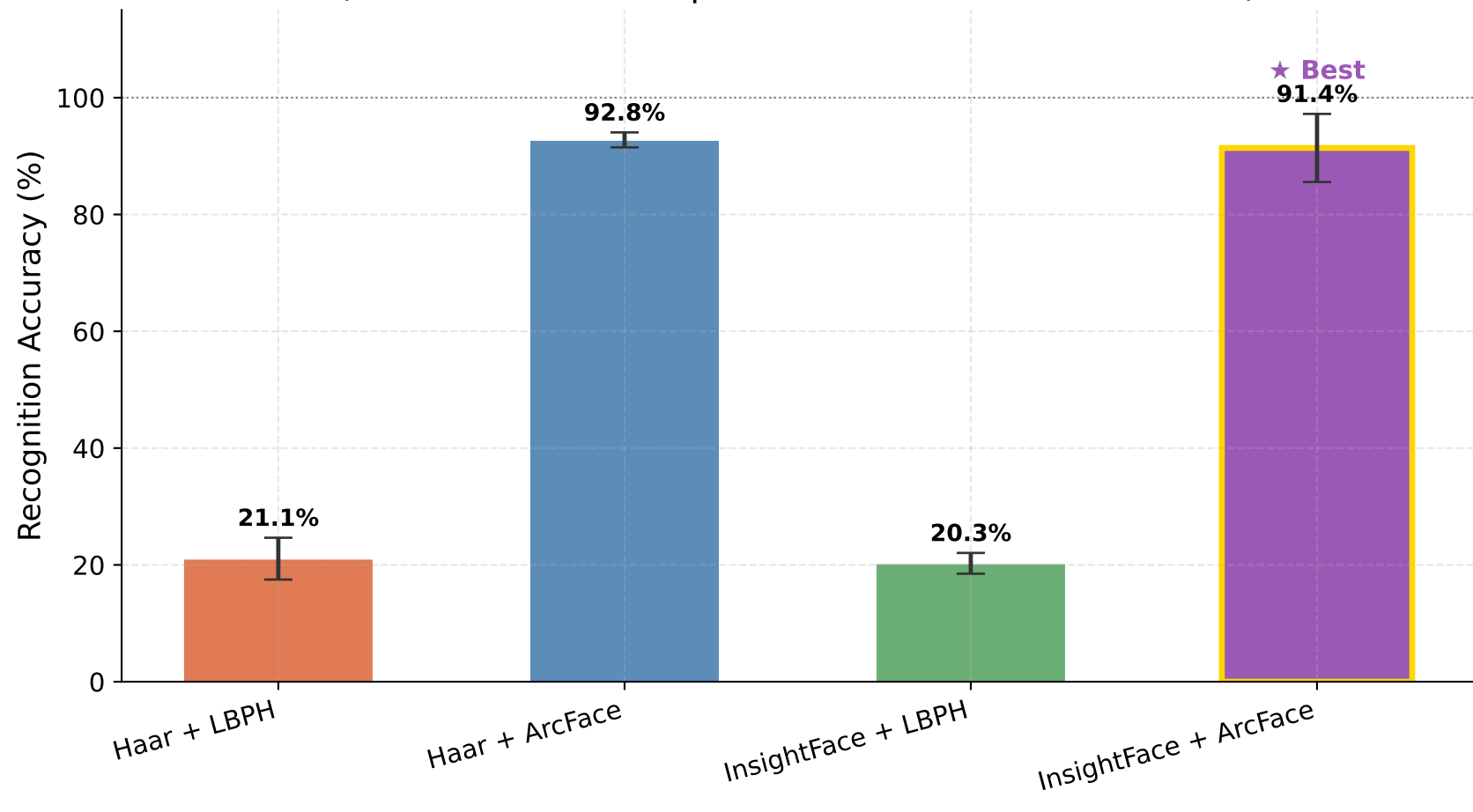
Recognition Accuracy Comparison (mean \pm std, 3 independent runs, threshold = 0.50)
