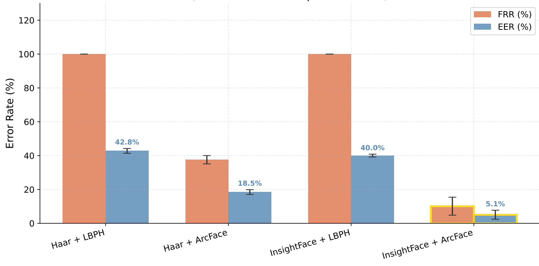
False Rejection Rate (FRR) and Equal Error Rate (EER) (mean \pm std, 3 independent runs)
