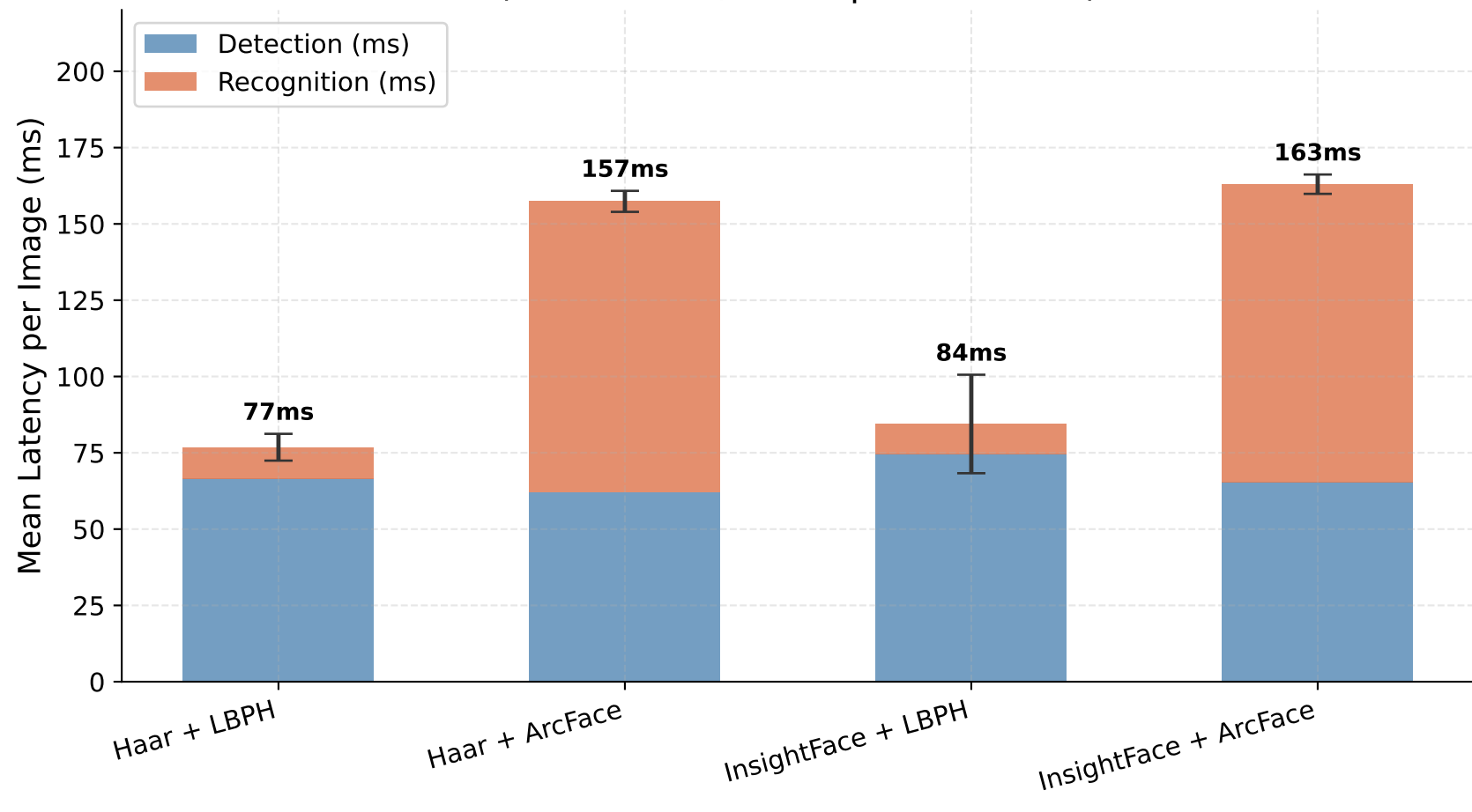
Pipeline Latency: Detection + Recognition (mean \pm std, 3 independent runs)
