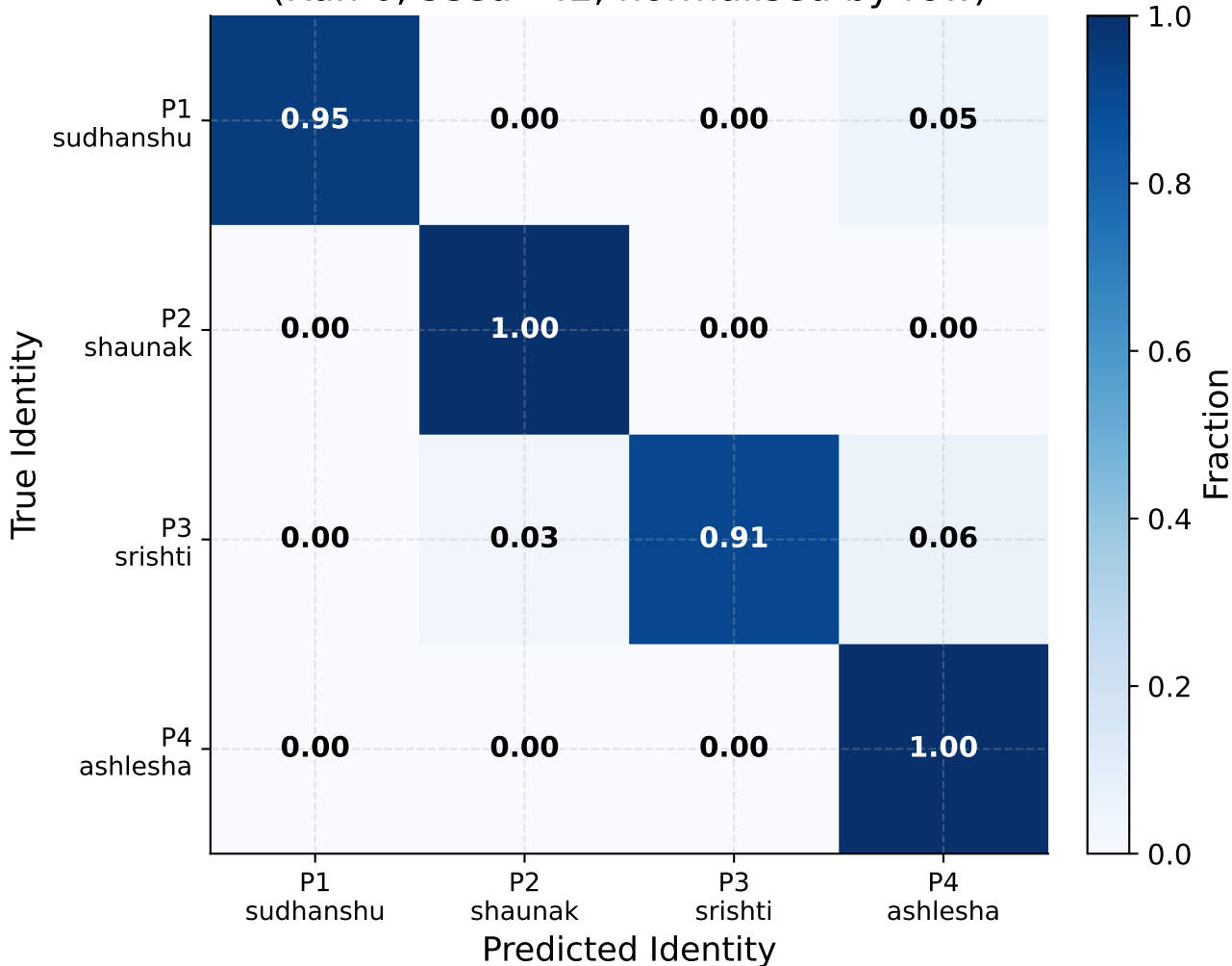
Confusion Matrix — InsightFace + ArcFace (Run 0, seed=42, normalised by row)
