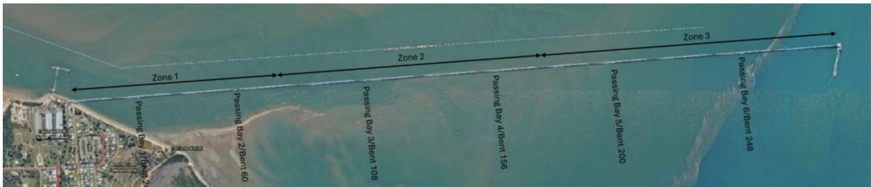
Figure 1. The jetty and its exposure zones. Zone 3 at the wharf head is open water and is worked first; the campaign finishes in the shelter of Zone 1.
