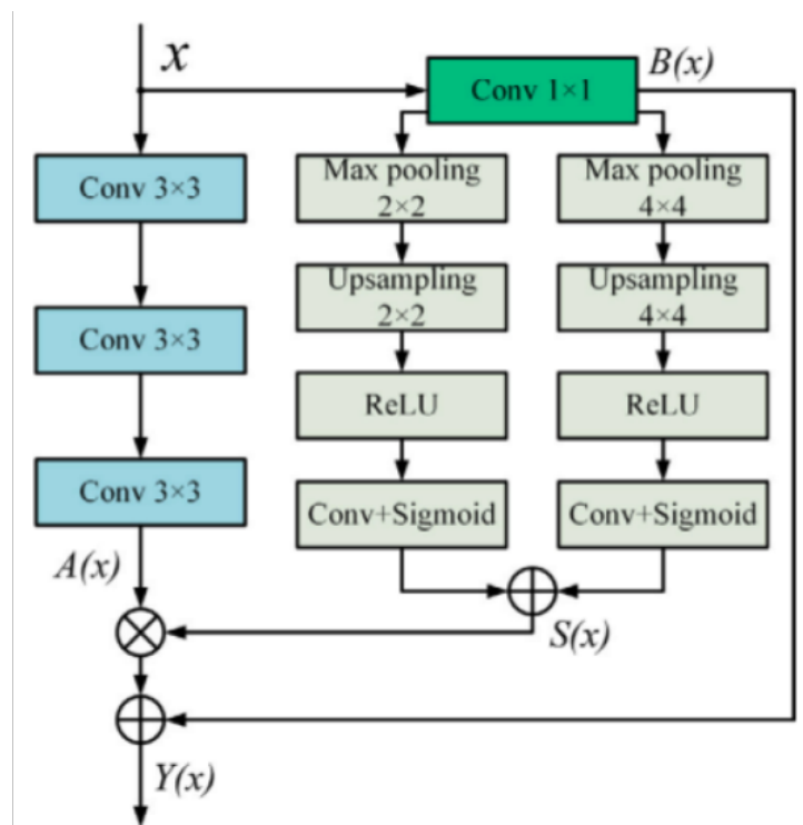
Figure 3.2: Diagram of the Spatial Attention Module (SAM) used in the AS-Net decoder. Adapted from K. Hu et al. (2022).
