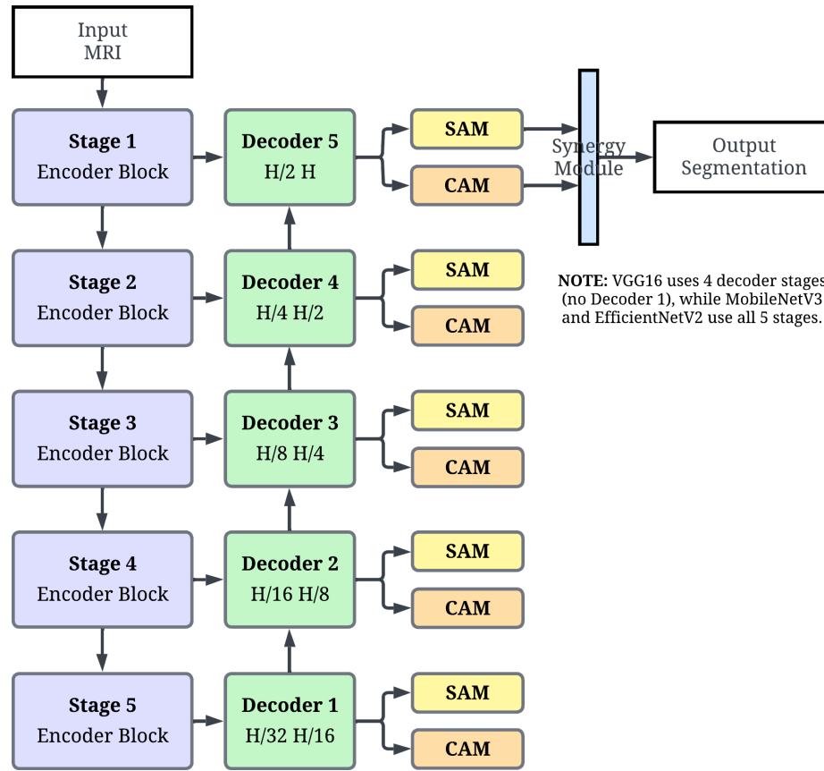
Figure 3.4: Complete AS-Net encoder-decoder architecture with attention modules.
