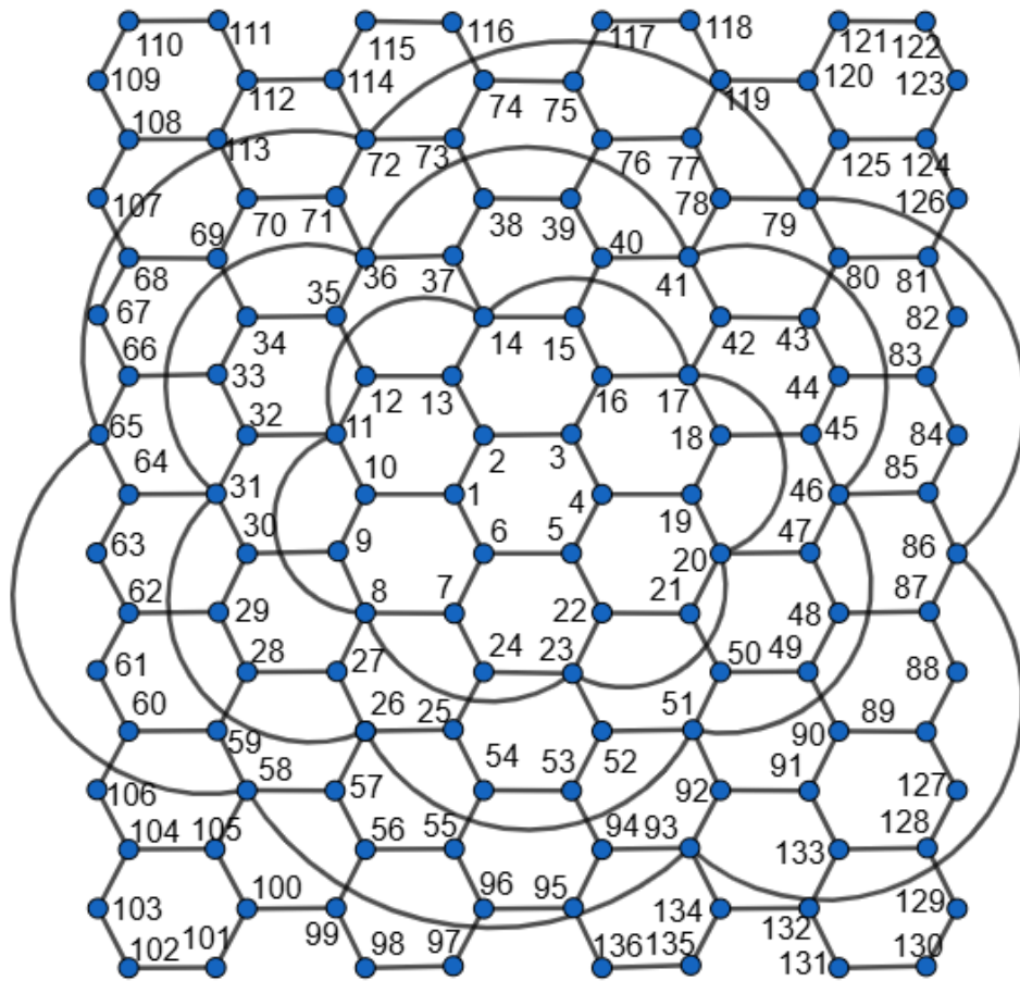
Enhanced Honeycomb rectangular mesh EHRM(8,9)
