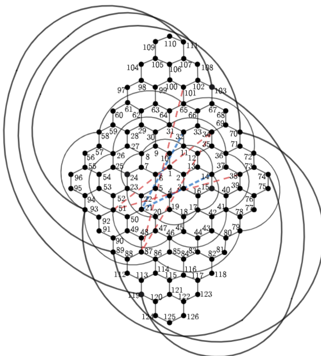
Enhanced Honeycomb Rhombic Mesh of type 2 EHRoM_2(8,8)
