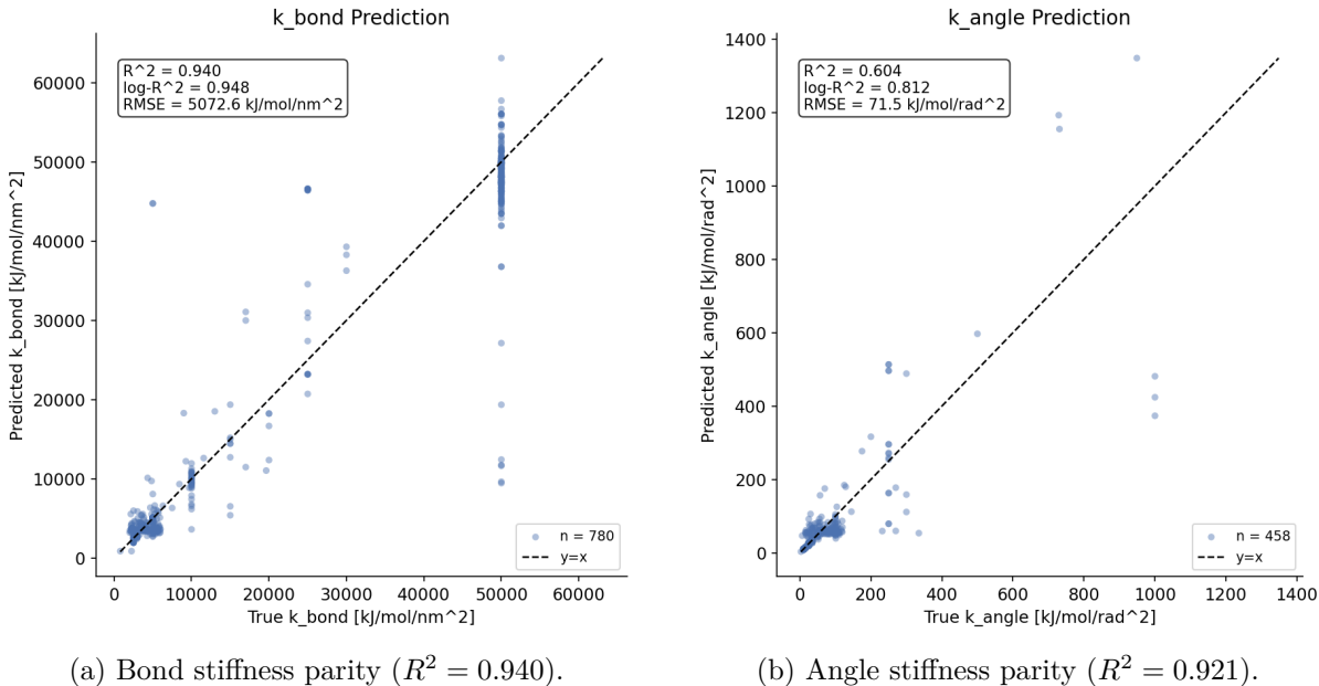
Figure 2: Parity plots comparing ground-truth versus predicted force constants across 122 held-out test molecules.
