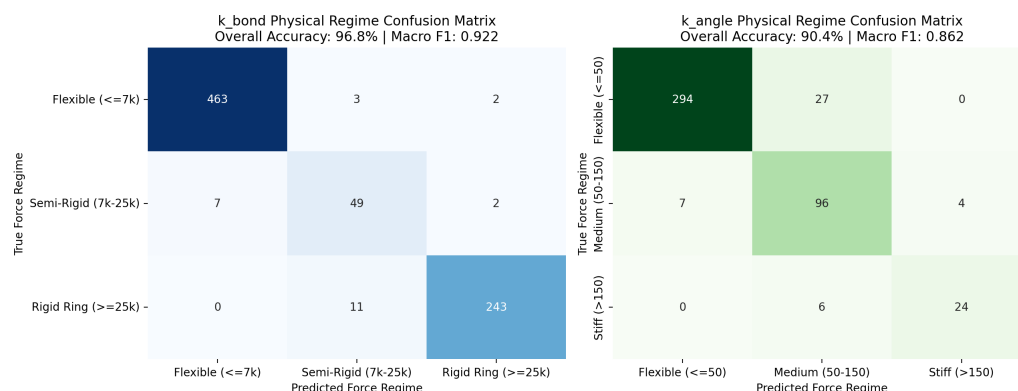
Fig. 5: Physical force regime confusion matrices for bond and angle spring constants, illustrating sharp diagonal dominance.
