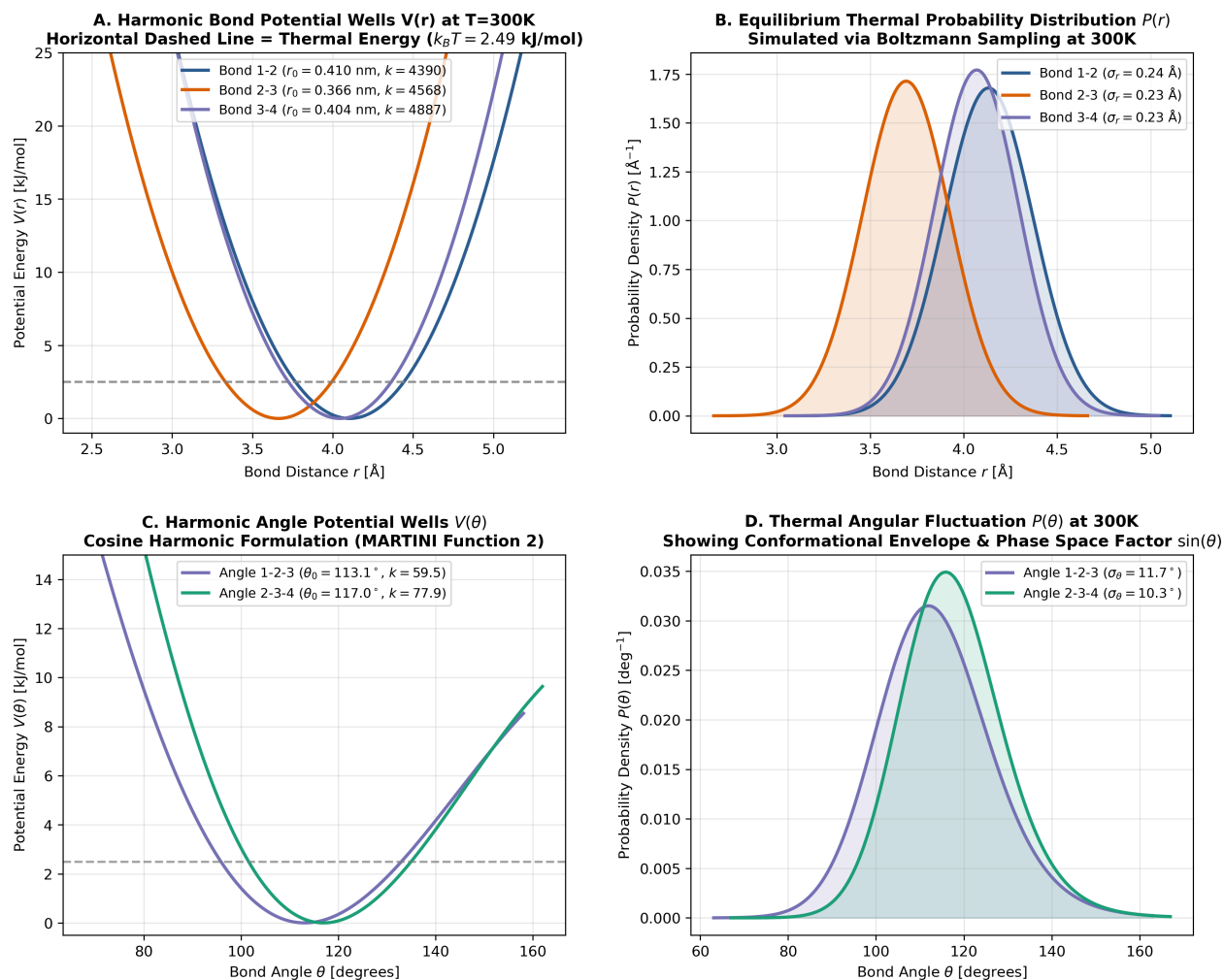
Fig. 7: Turnkey parameterization and physical verification diagnostic for Coarse-Grained Ibuprofen (IBUP).
