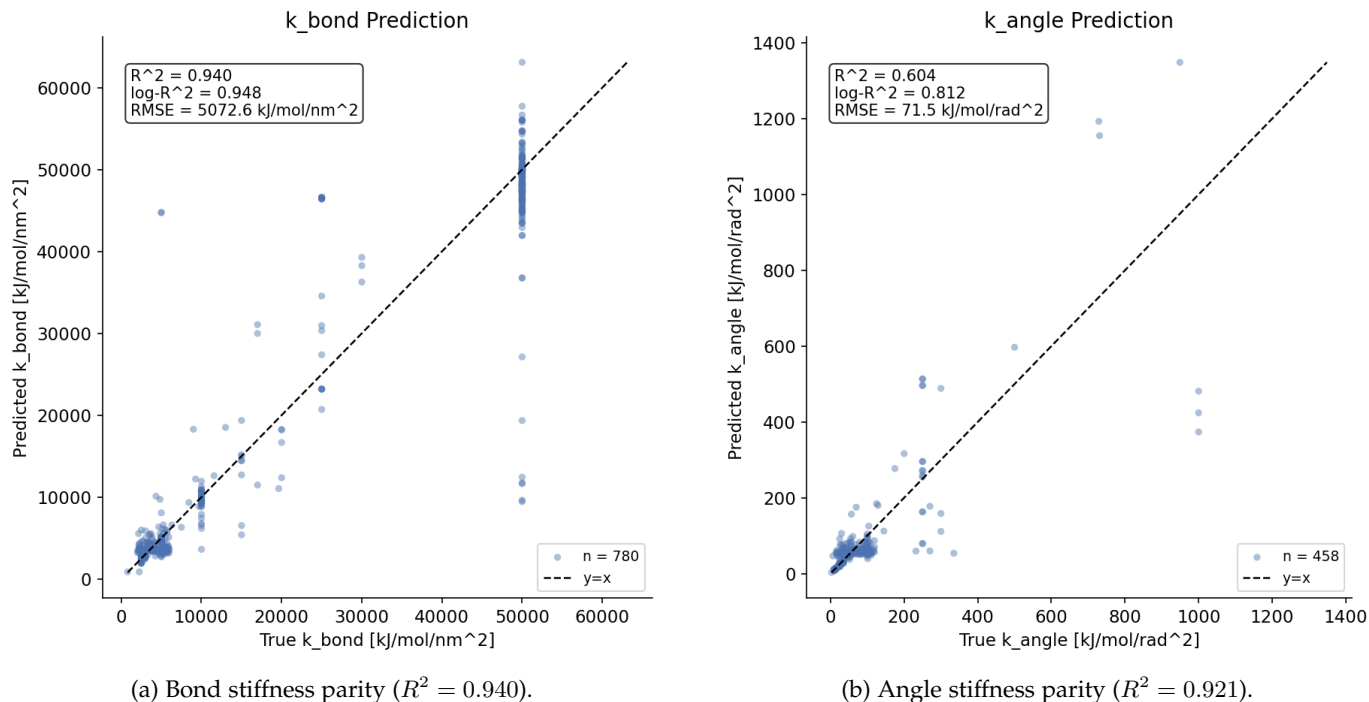
Fig. 2: Parity plots comparing ground-truth versus predicted force constants across 122 held-out test molecules.
