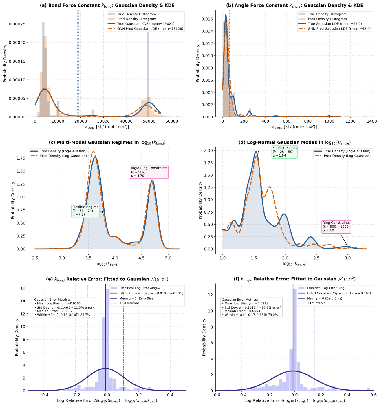
Fig. 4: Six-panel Gaussian density and homoscedastic error bell curve analysis for bond and angle force constants.
