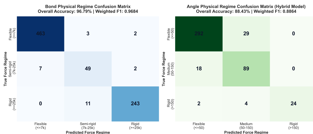
Fig. 5: Physical force regime confusion matrices for bond and angle spring constants, illustrating sharp diagonal dominance.
