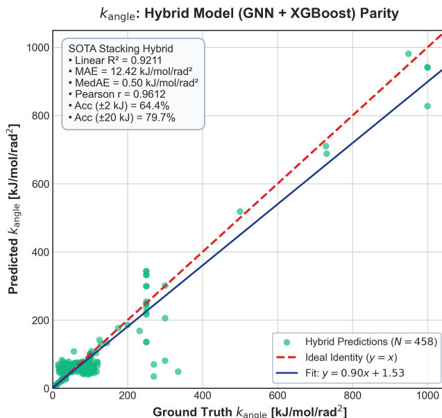
(b) Angle stiffness parity ( R^2 = 0.921 ).
