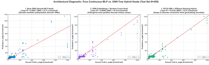
Fig. 1: Architectural diagnostic comparing the smooth continuous manifold of the pure GNN against the orthogonal decision boundary partitioning of the Stacking Hybrid Model.
