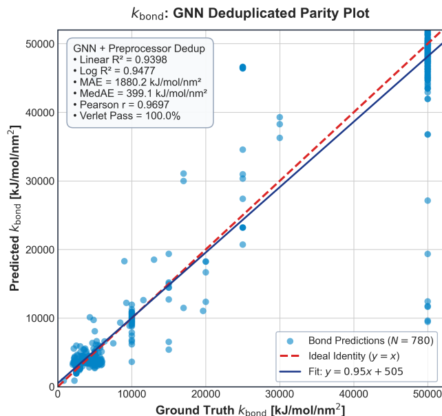
(a) Bond stiffness parity ( R^2 = 0.940 ).
