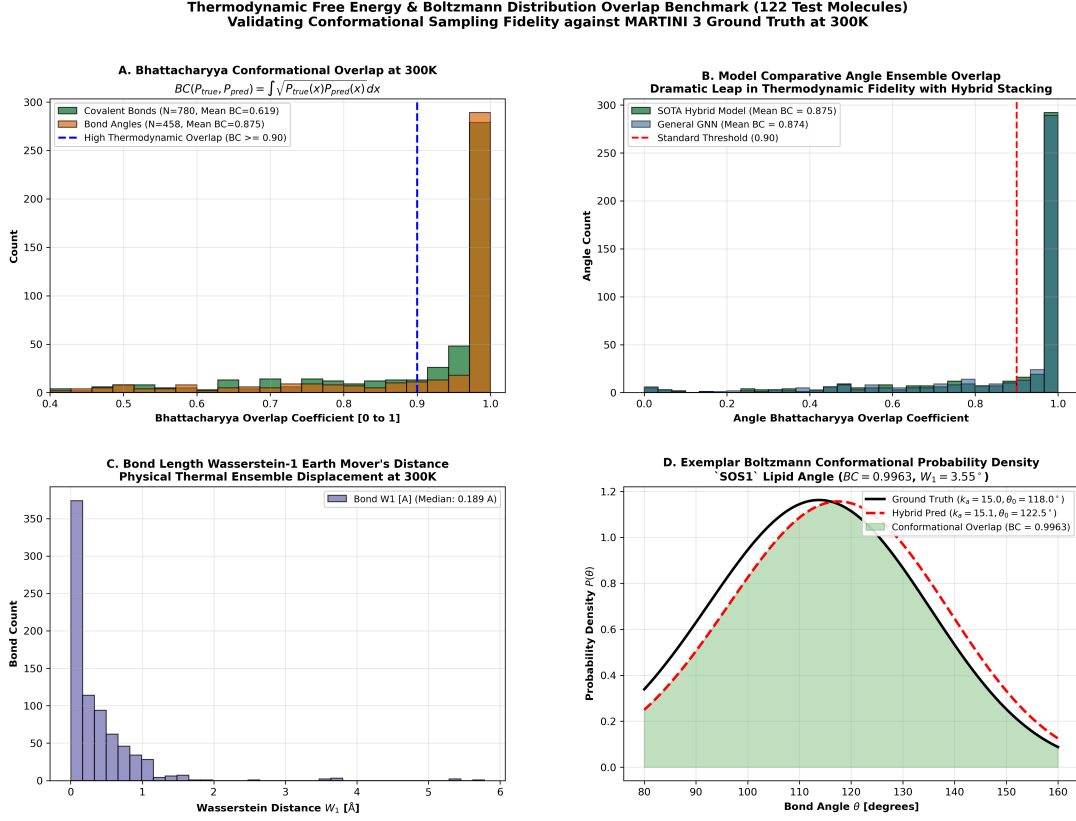
Figure 6: Thermodynamic Boltzmann distribution overlap benchmark at 300 K, demonstrating 99.5% median conformational overlap ( BC = 0.9948 ).
