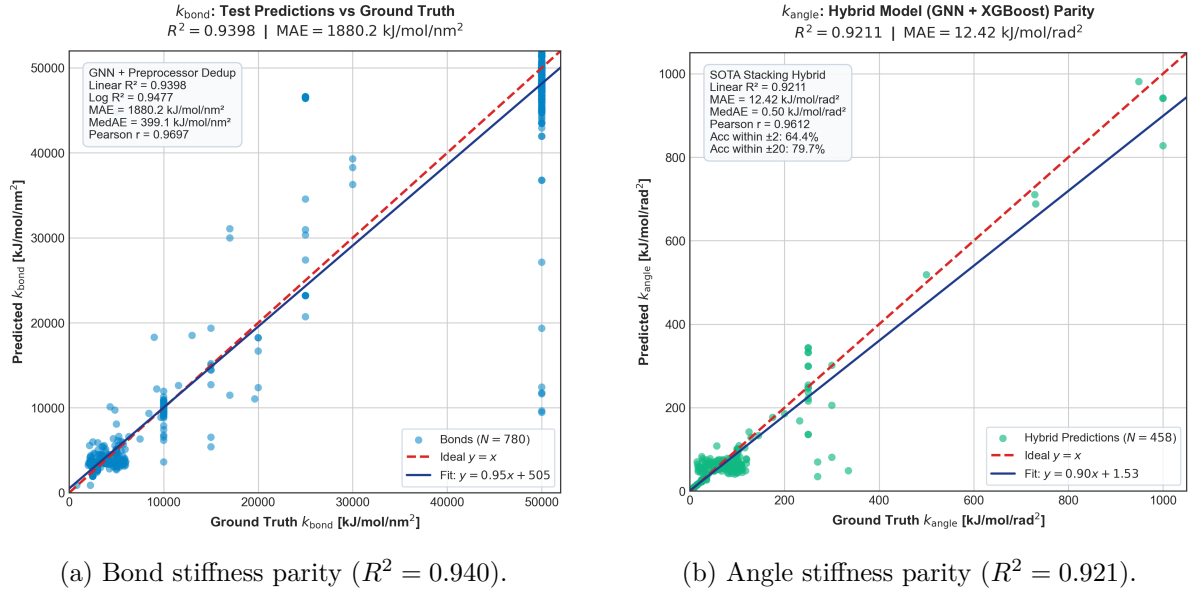
Figure 2: Parity plots comparing ground-truth versus predicted force constants across 122 held-out test molecules.
