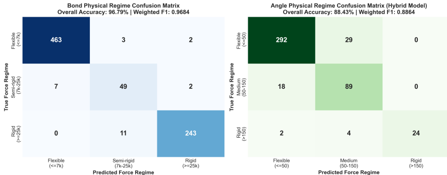
Figure 5: Physical force regime confusion matrices for bond and angle spring constants, illustrating sharp diagonal dominance.
