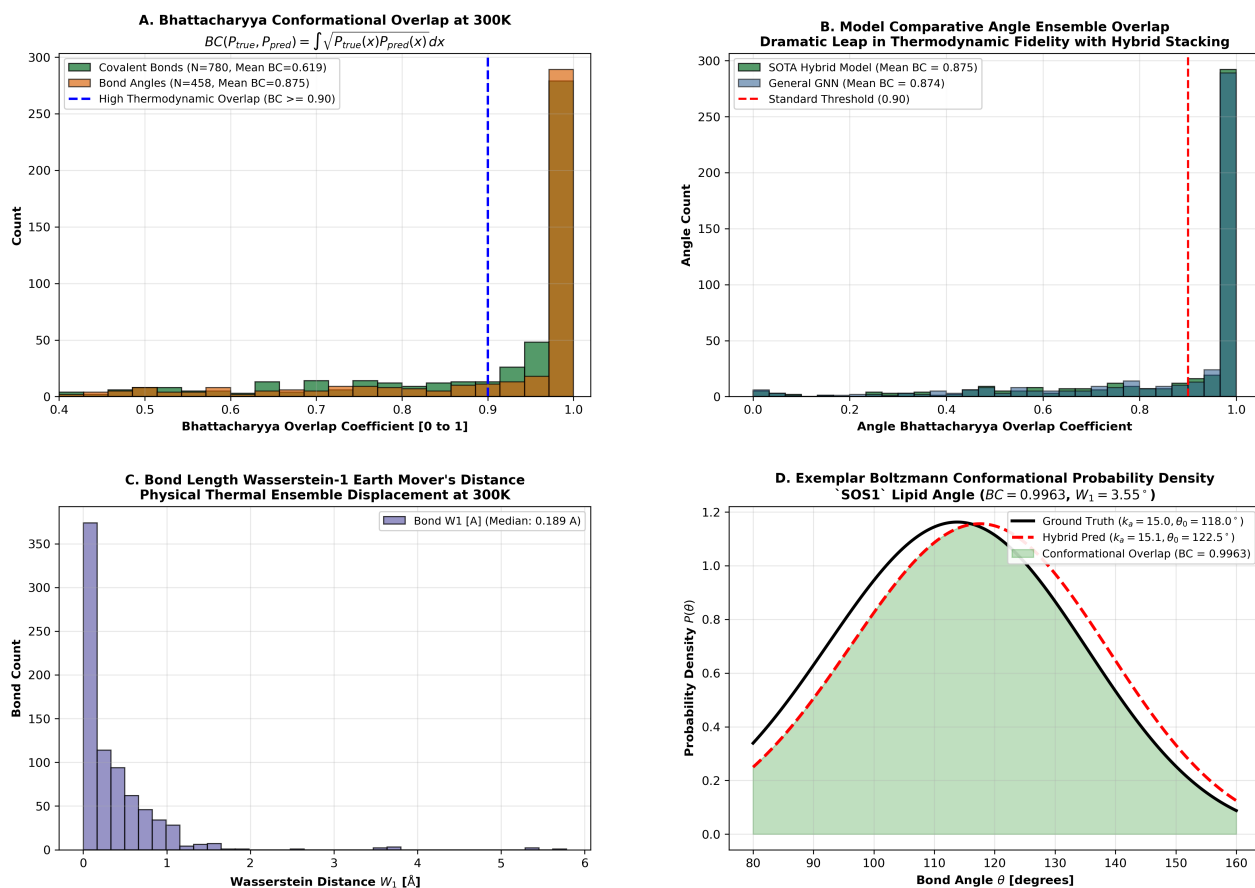
Fig. 6: Thermodynamic Boltzmann distribution overlap benchmark at 300 K, demonstrating 99.5% median conformational overlap ( BC = 0.9948 ).
