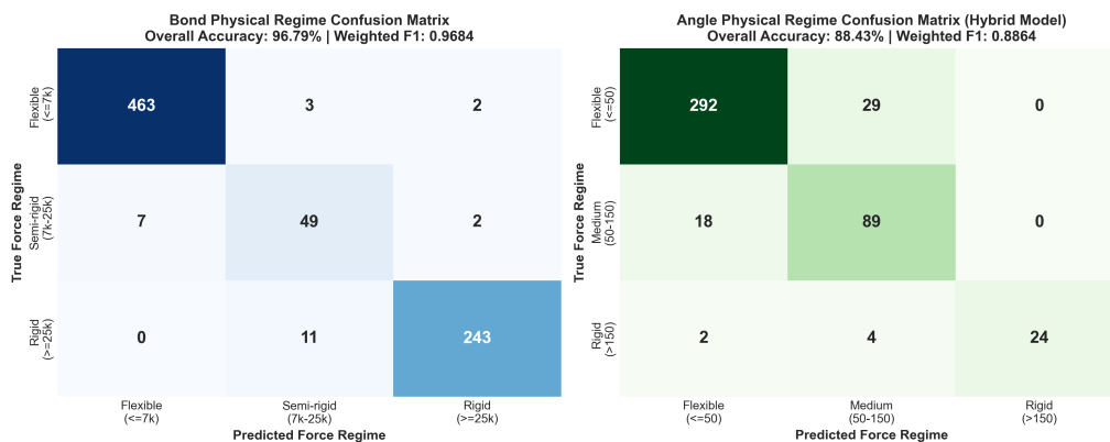
Fig. 5: Physical force regime confusion matrices for bond and angle spring constants, illustrating sharp diagonal dominance.
