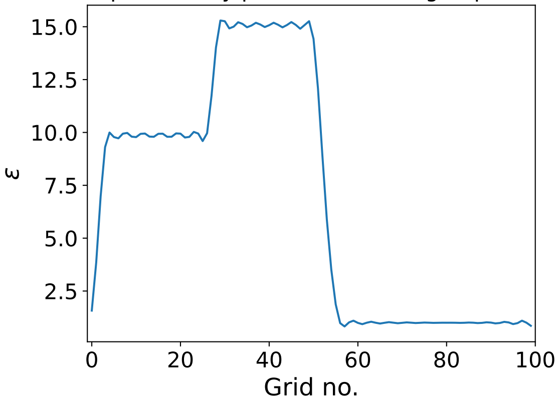
TORCWA permittivity profile. n_G = 12 , grid points = 100
