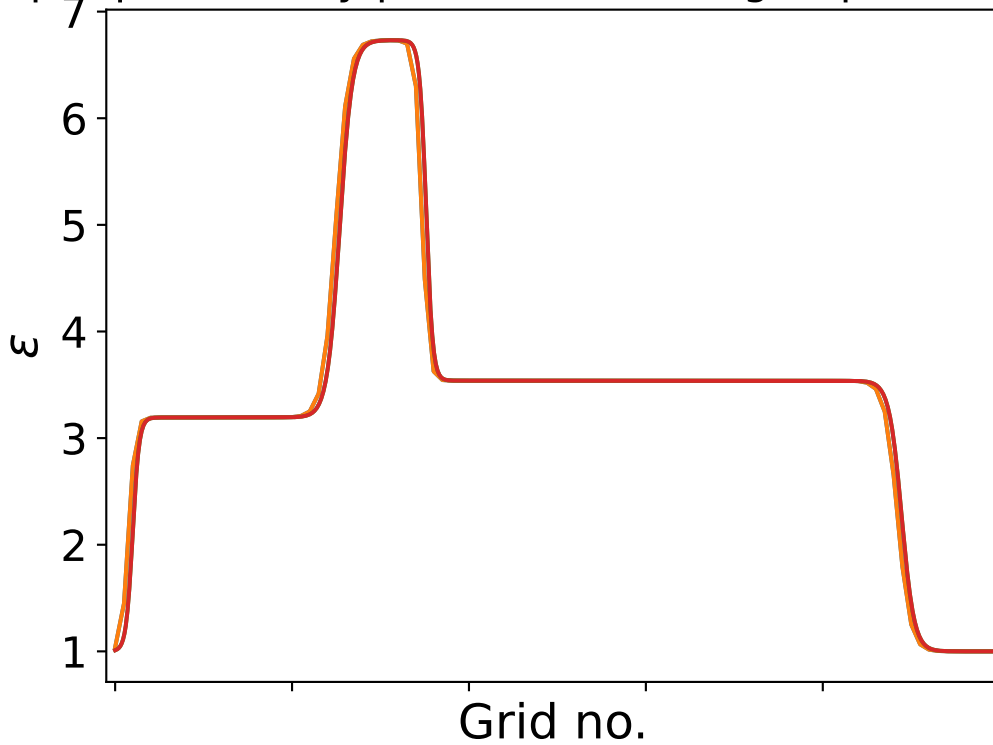
TORCWA permittivity profile. n_G = 12 , grid points = 100
