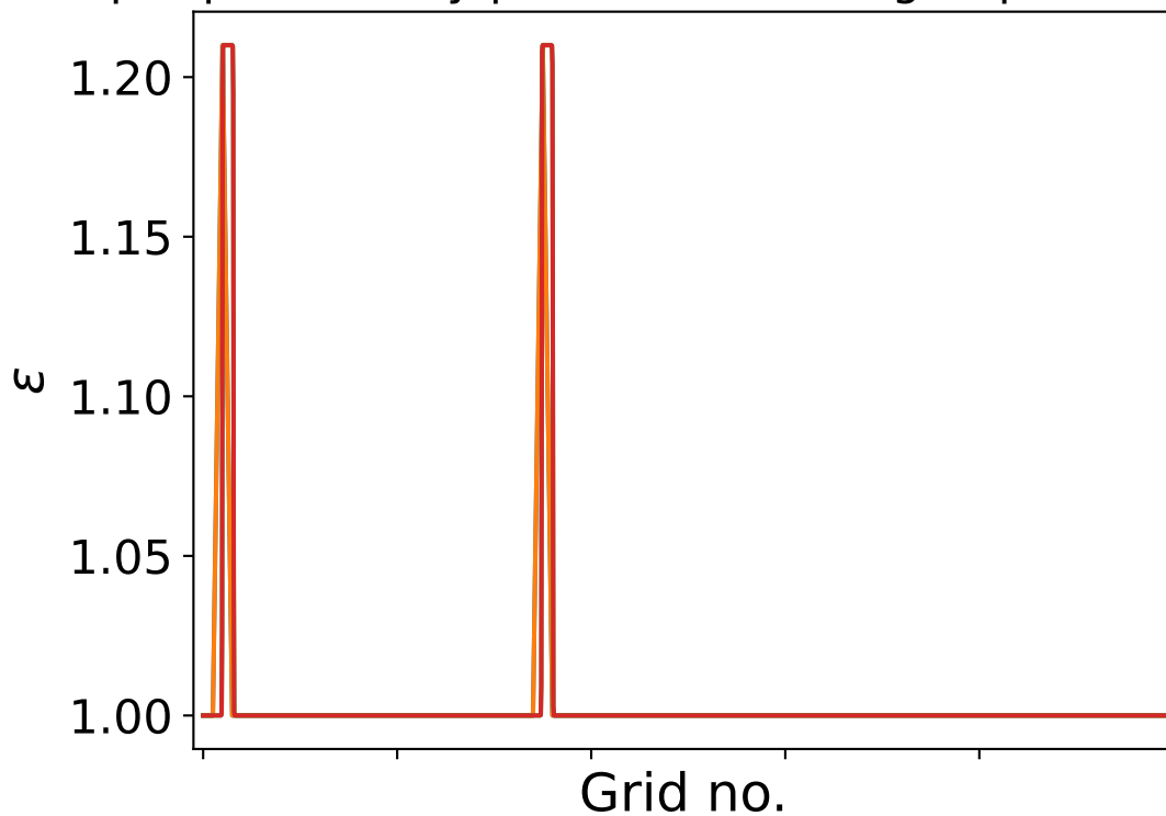
TORCWA permittivity profile. n_G = 12 , grid points = 100
