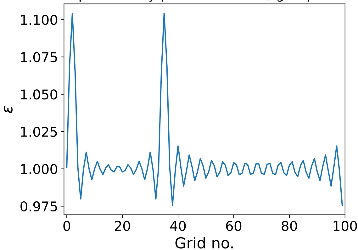
TORCWA permittivity profile. n_G = 12 , grid points = 100
