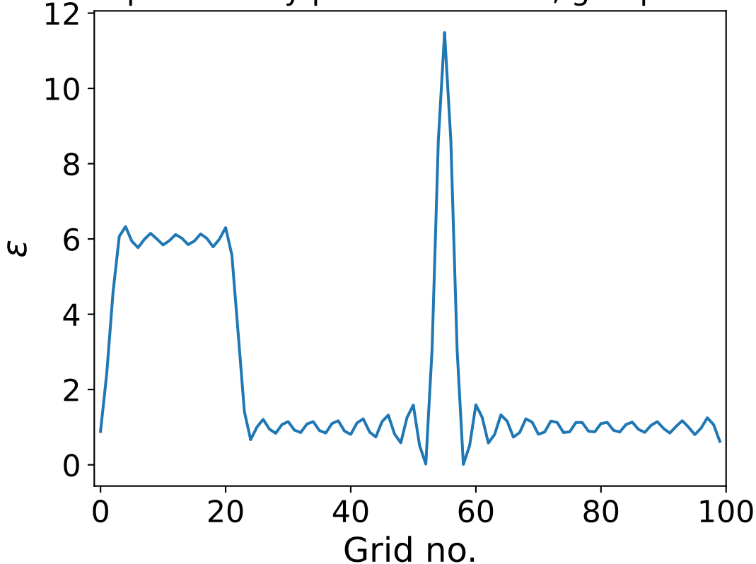
TORCWA permittivity profile. nG = 12, grid points = 100
