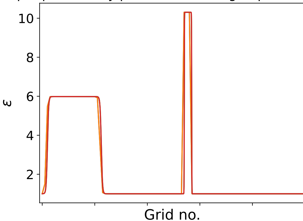
TORCWA permittivity profile. nG = 12, grid points = 100
