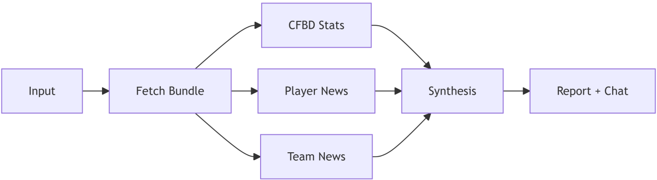
Transfer Portal Architecture
