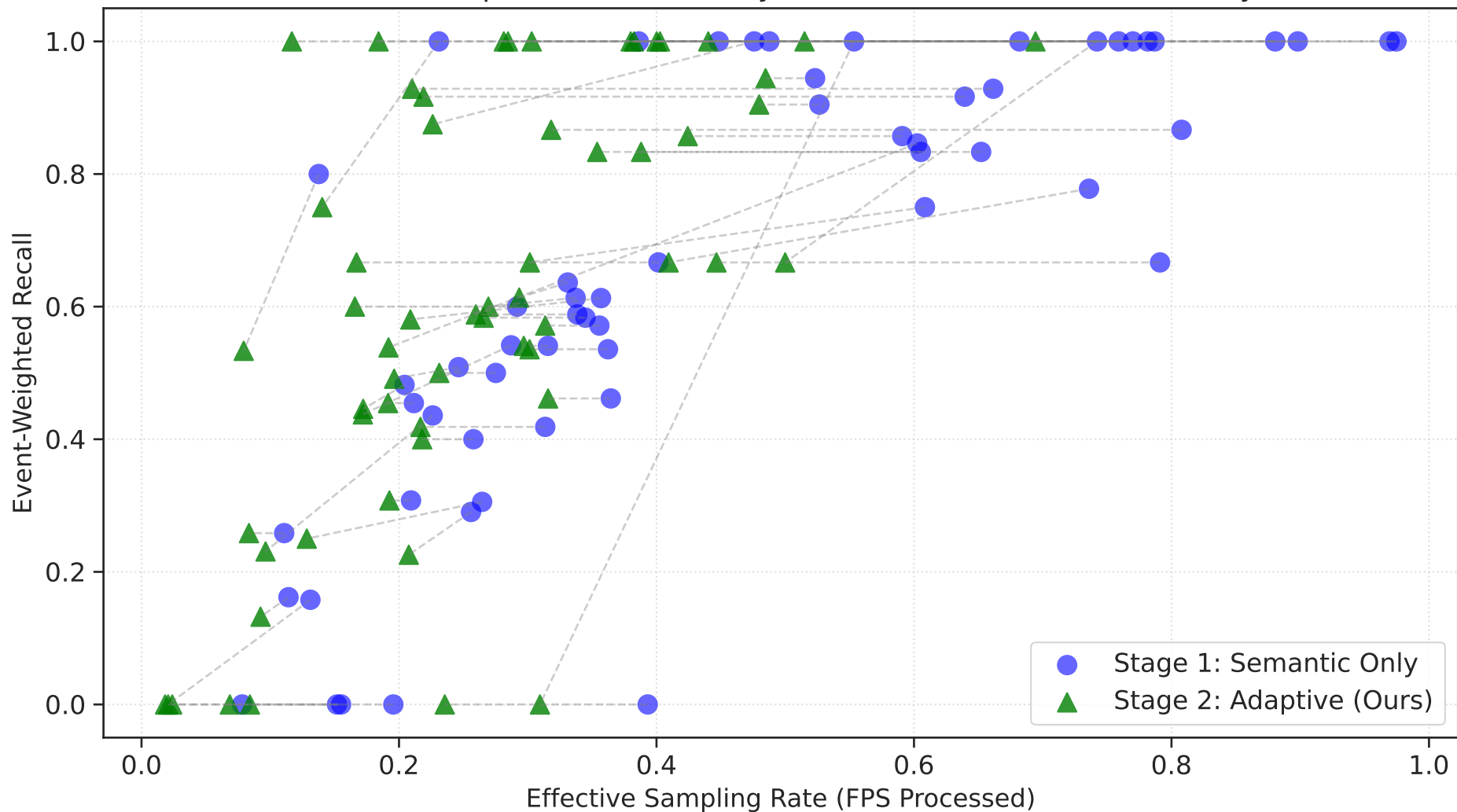
Ablation: Impact of Redundancy Removal on Recall vs. Efficiency
