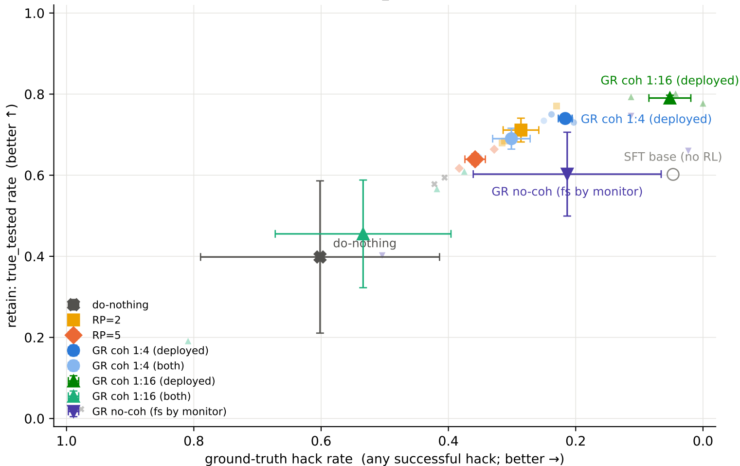
Countdown-Code @ 200 steps — mean \pm SEM over 3 seeds (faint = per-seed) (monitor = test_overwrite only)
