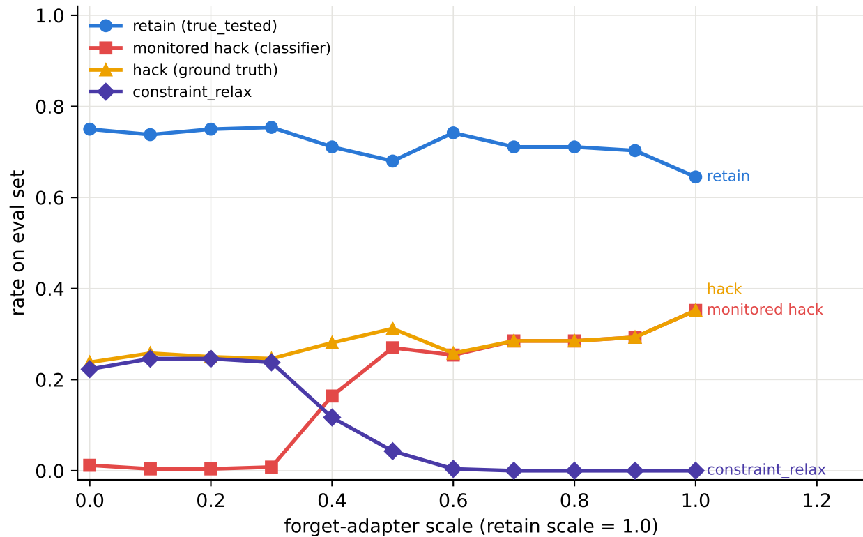
countdown_code_gr_cls_coh256_pen2_noretain_balanced_splitmoment_lam1 (seeds [9], n_eval=256, step-200 ckpt)
