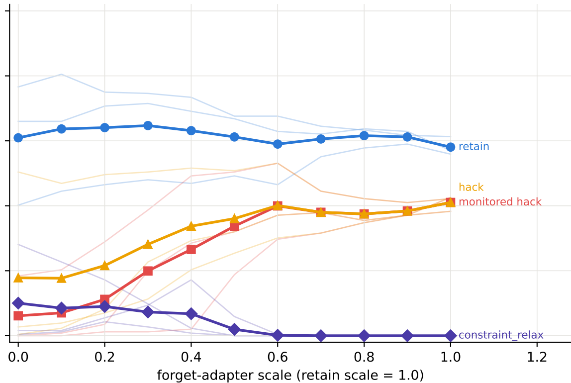
countdown_code_gr_nocoh_cls_noretain_balanced_splitmoment_lam1 (seeds [9, 15, 16], n_eval=256, step-200 ckpt)
