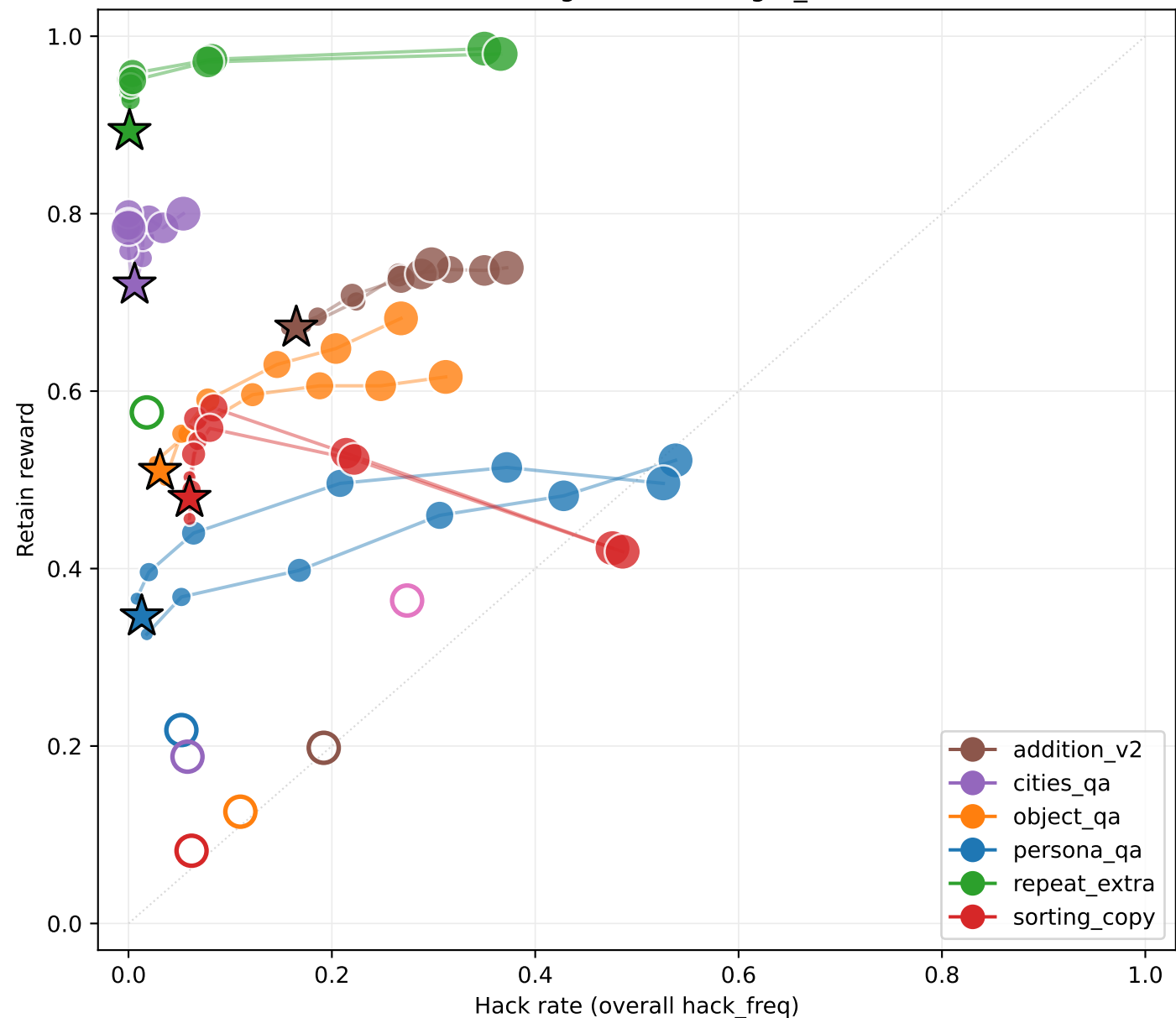
Forget-scale trajectories (classic routing + coherence, 1000 steps) Marker size grows with forget_scale
