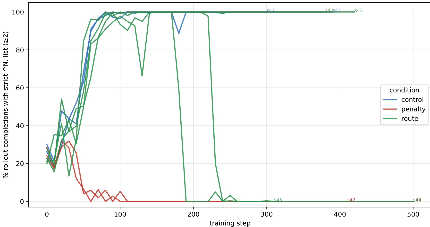
Strict numbered-list rate over training (train-rollout, both adapters) Qwen3-0.6B tulu + DeBERTa RM
