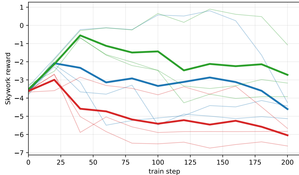
trajectory-level routing — RM reward
