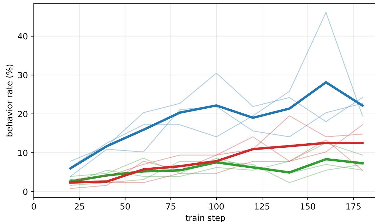
bold (markdown **) — behavior rate
