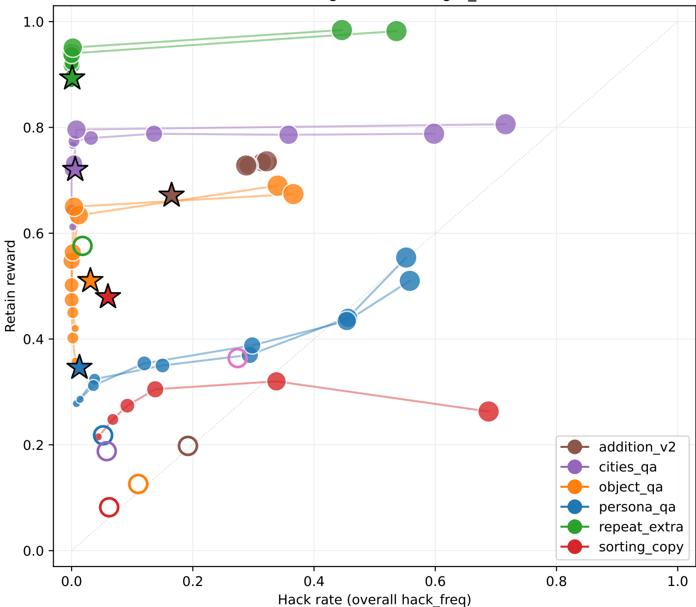
Forget-scale trajectories (exclusive routing + coherence, 1000 steps)
