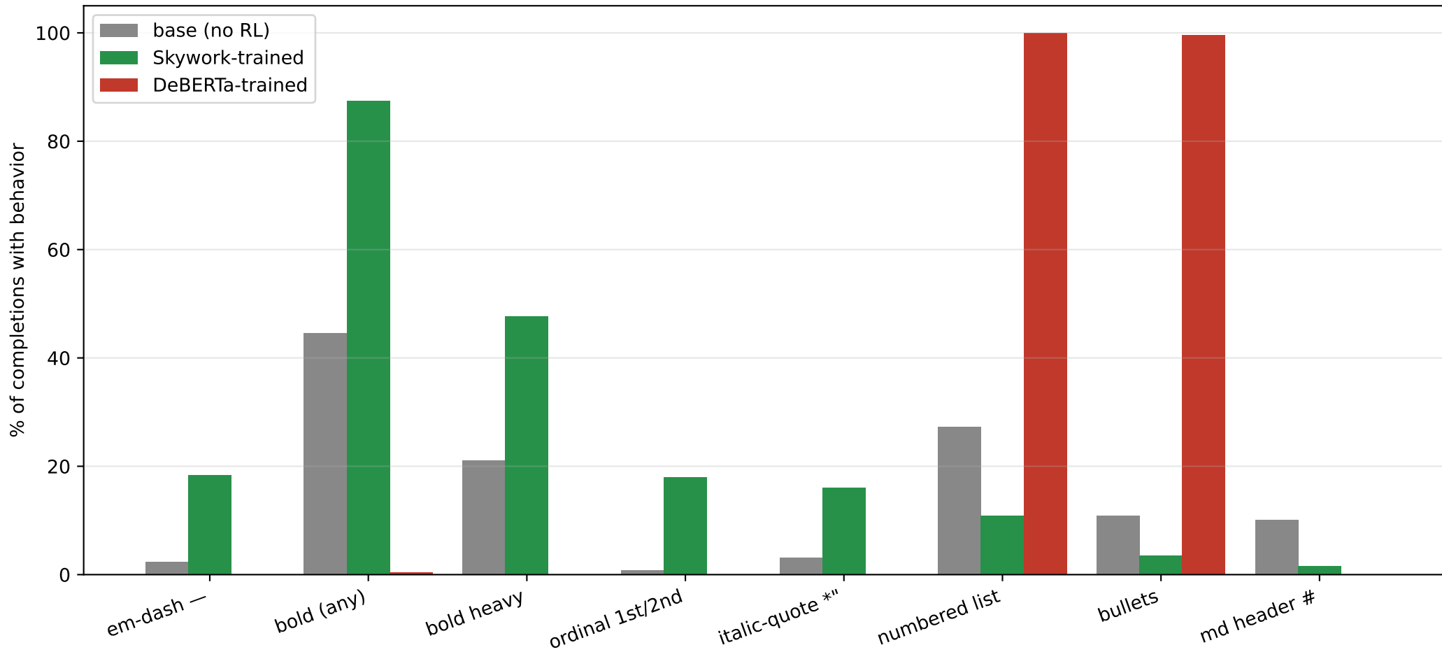
Behaviors taught by the reward model (per-completion rate vs base) Qwen3-0.6B tulu, 256 matched eval prompts
