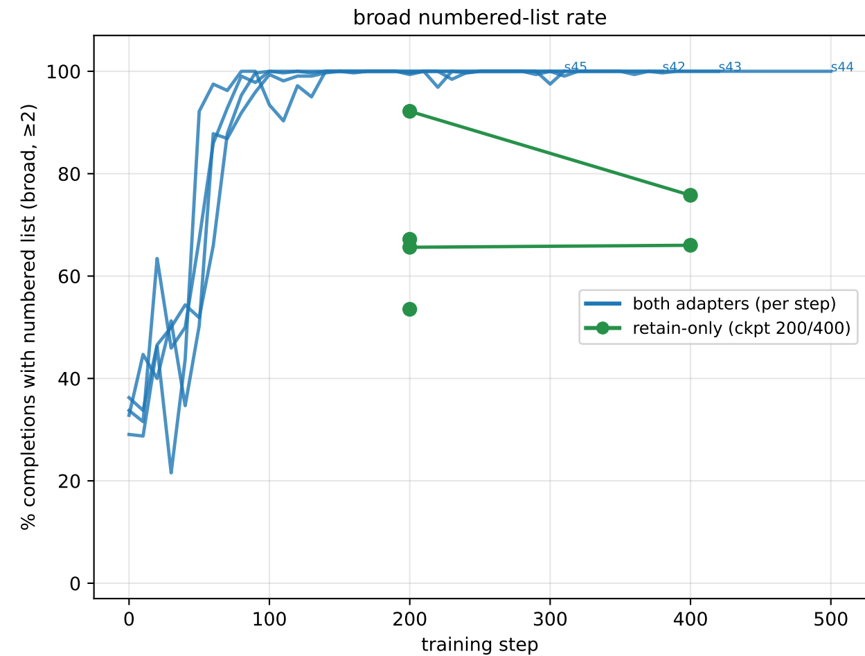
Routing seeds: forget-ablation costs reward — list rate (left) vs RM score (right), Qwen3-0.6B tulu
