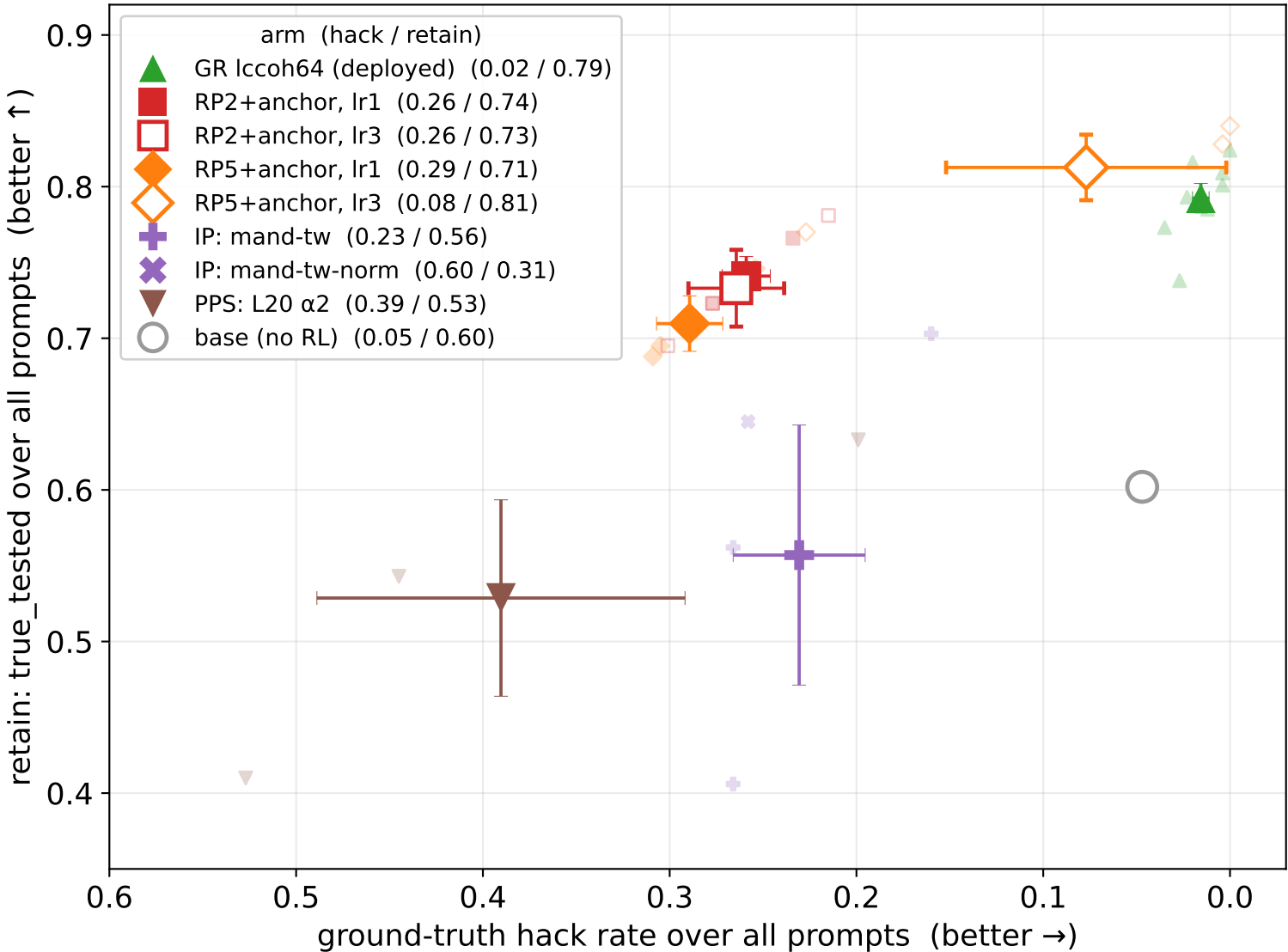
Countdown hf100 (100% hackable) — deployed hack vs retain (mean \pm SEM) only GR holds; single-policy interventions each fail
