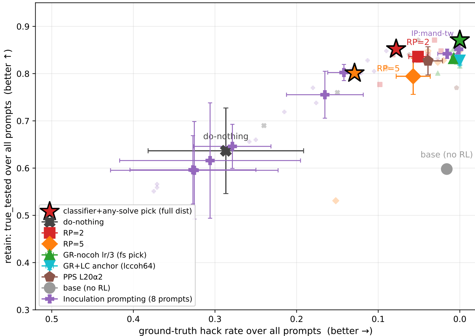
Countdown hf50 (50/50 hackable) — deployed hack vs retain (mean \pm SEM) IP: 8 train-time prompts, deployed prompt-removed; GR-nocoh fs classifier-selected; faint = per-seed
