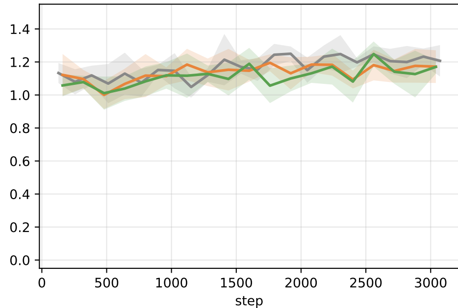
retain reward
