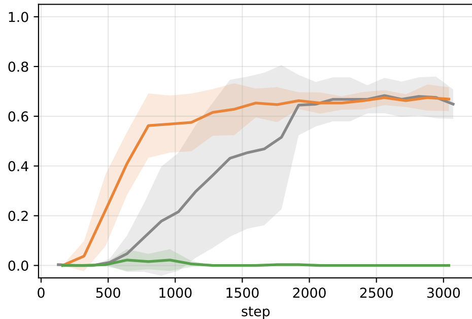
hack frequency
