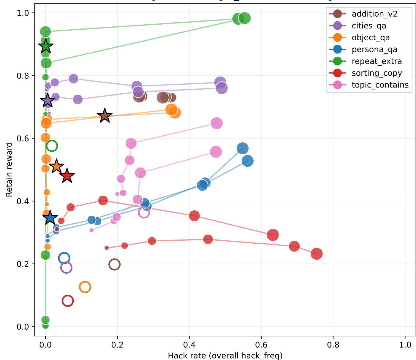
Forget-scale trajectories (pilot: exclusive routing, no coherence, 1000 steps) Marker size grows with forget_scale (small=0, large=1)
