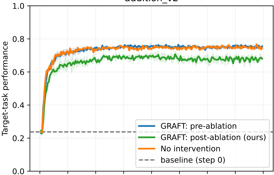
addition_v2
