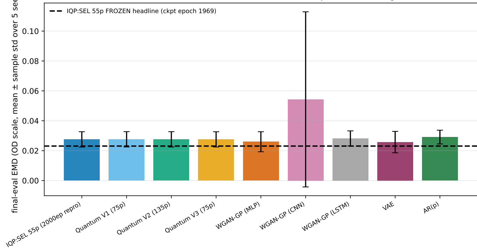
Cross-model final-eval EMD (OD scale, 2000ep matched budget)
