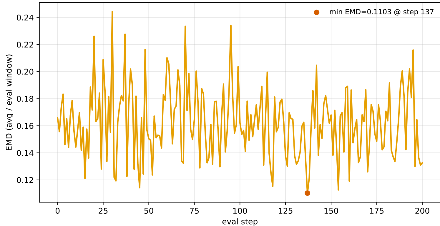
EMD over training — Quantum V3 (75p)
