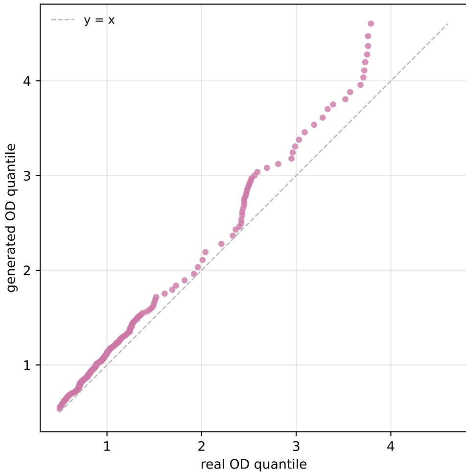
Q-Q plot — WGAN-GP (CNN)
