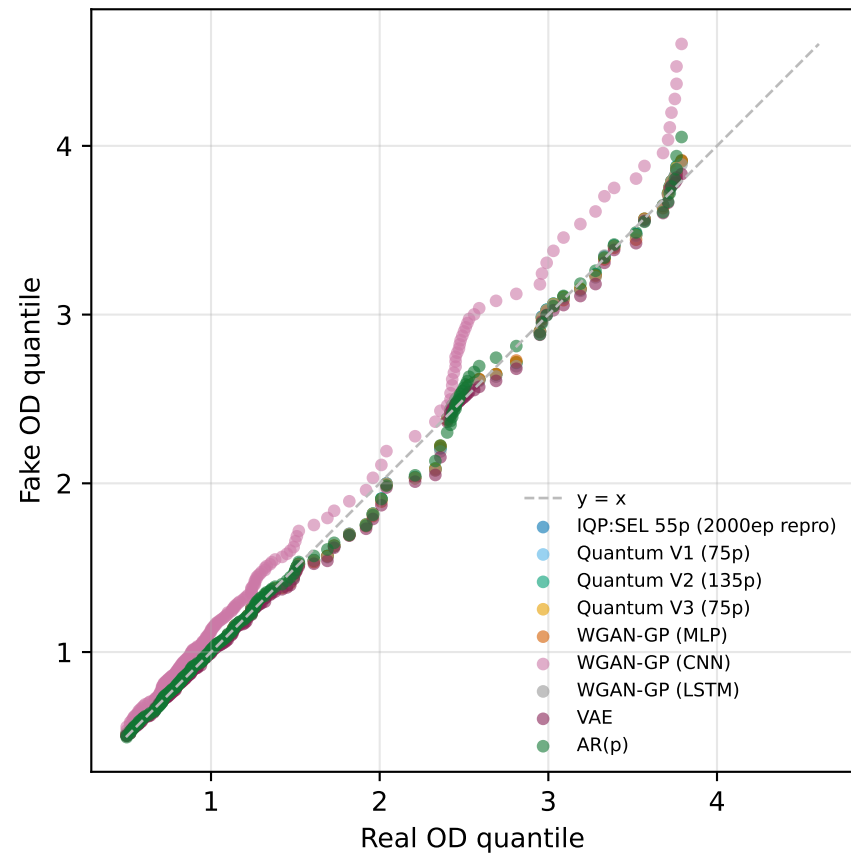
(a) QQ overlay — all 9 models on shared axes
