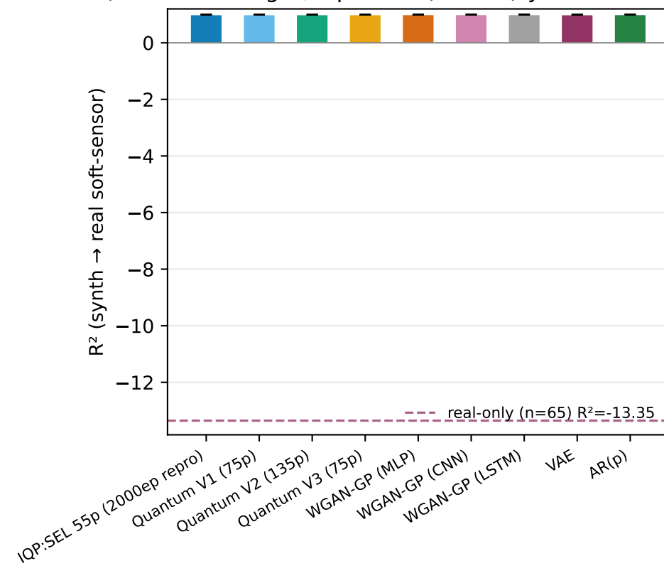
TSTR (matched-budget, Pipeline B) — R^2 (synth \rightarrow real soft-sensor)
