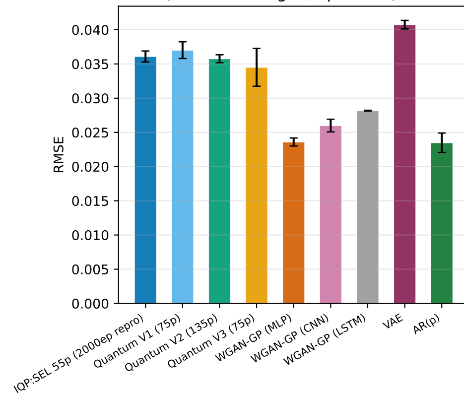
TSTR (matched-budget, Pipeline B) — RMSE
