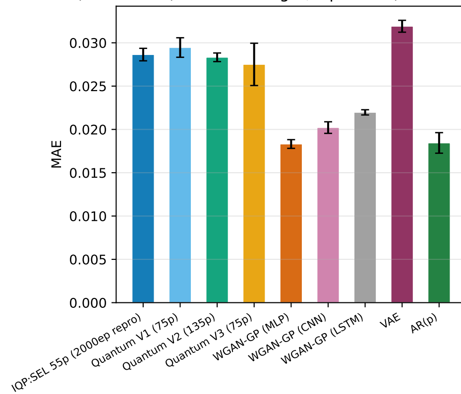
TSTR (matched-budget, Pipeline B) — MAE
