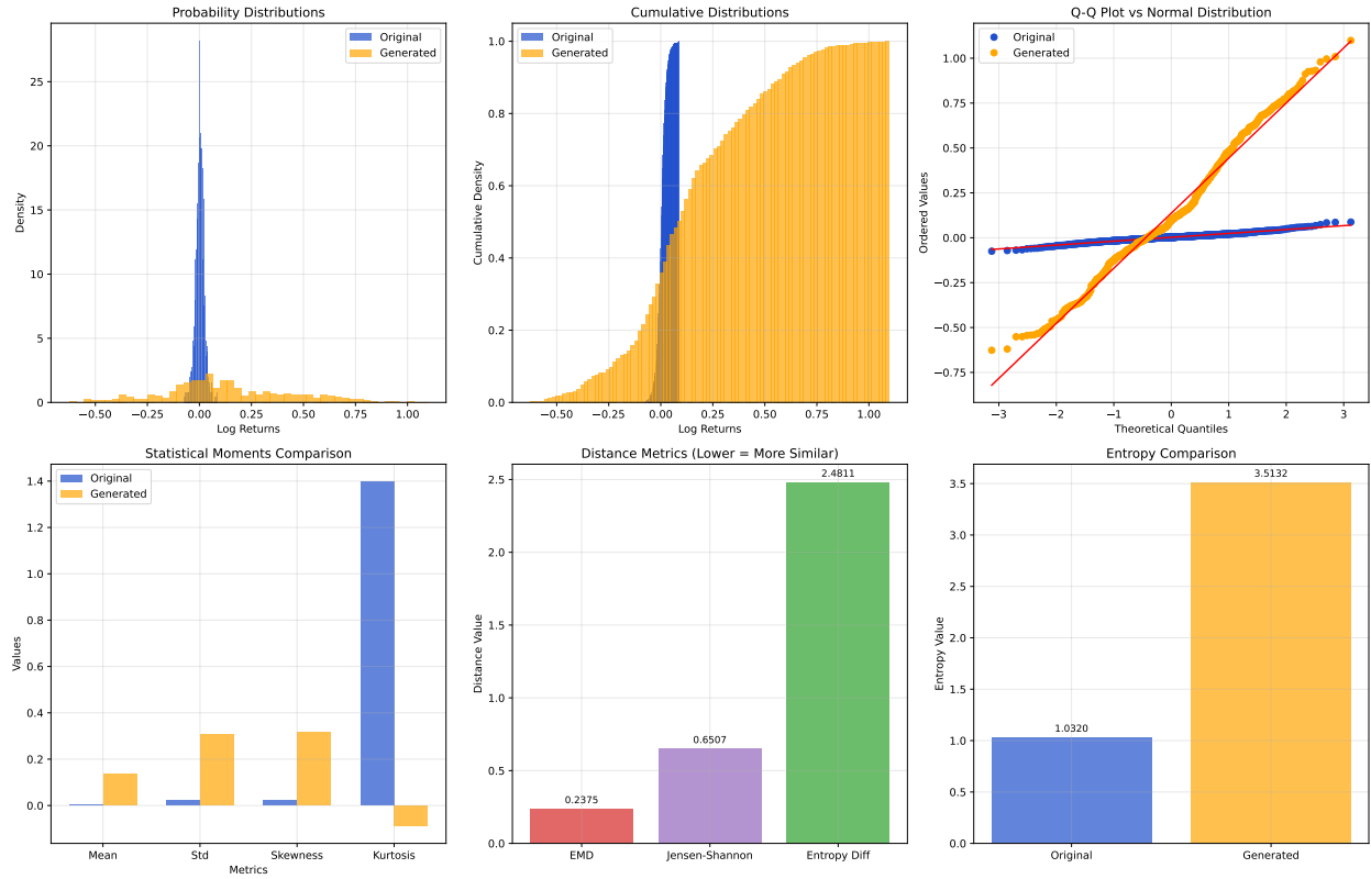
Figure A21: Log-return distribution diagnostics: WGAN-GP (CNN, 73p), seed 42 (the OD-EMD outlier seed disclosed in main-text §4.1). Panels as in Figure A16.
