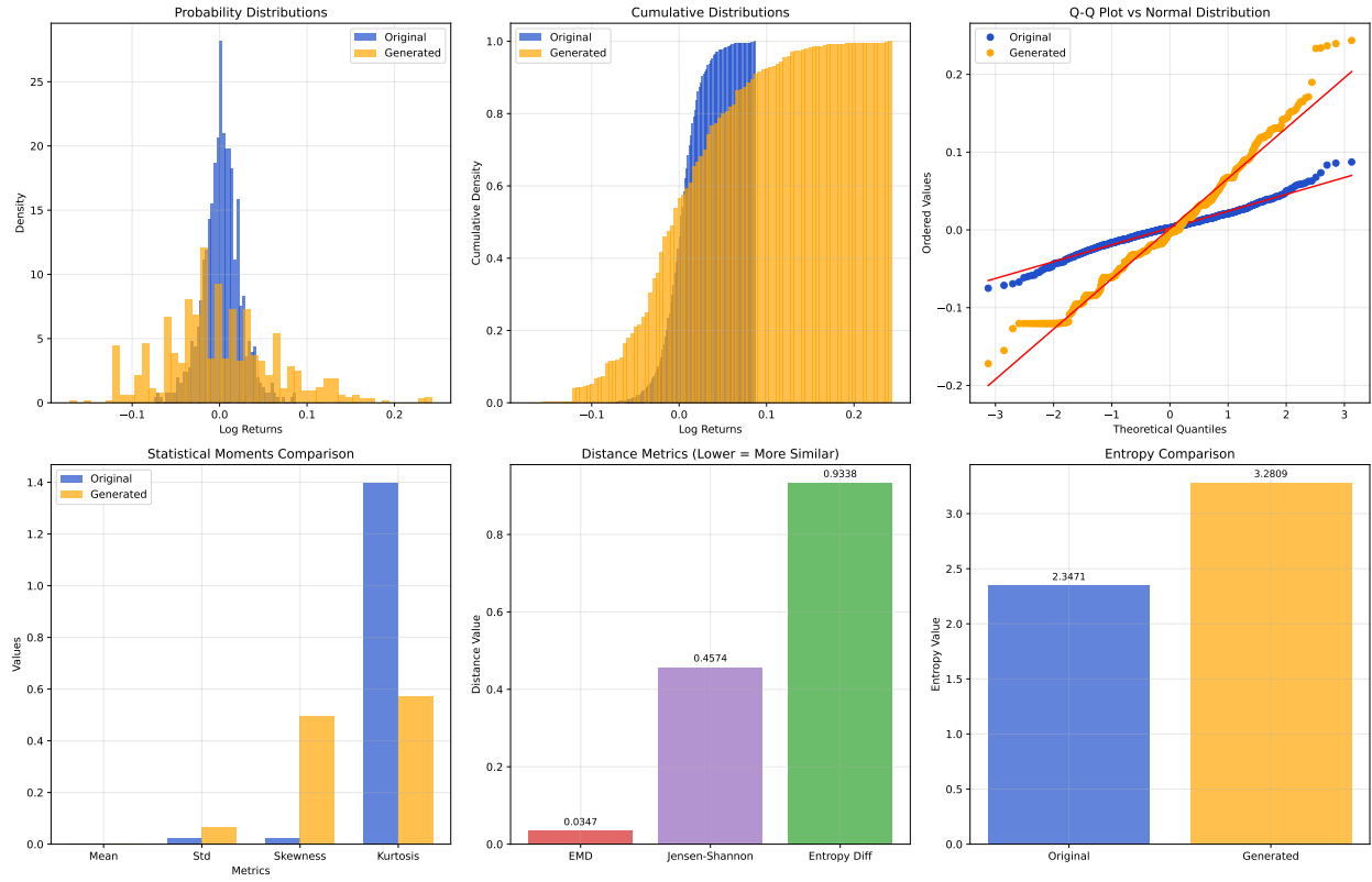
Figure A20: Log-return distribution diagnostics: WGAN-GP (MLP, 74p), seed 42. Panels as in Figure A16.
