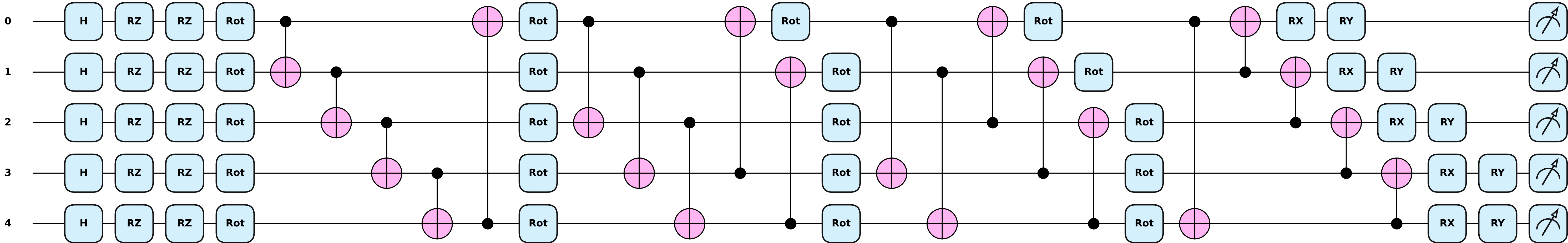
V1 - 5 qubits x 4 layers x range topology - 75 parameters
