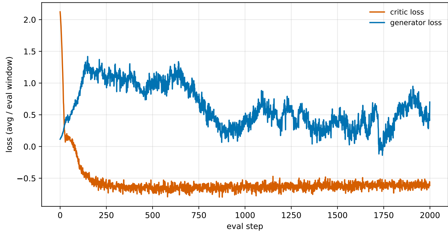
Training/fit curve — WGAN-GP (MLP)
