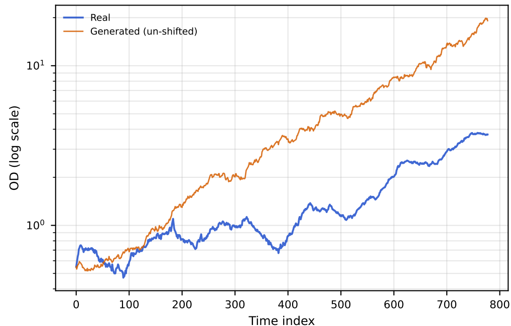
WGAN-GP (CNN) [C] — per-step bias +0.1345; compound \sim 2e+45\times overshoot
