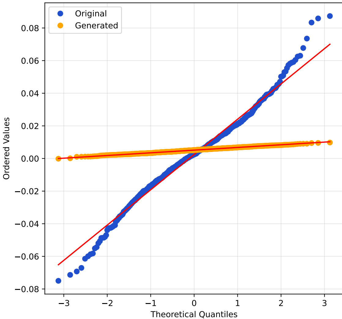
Entropy Comparison
