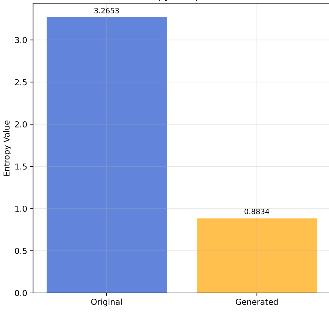
Entropy Comparison
