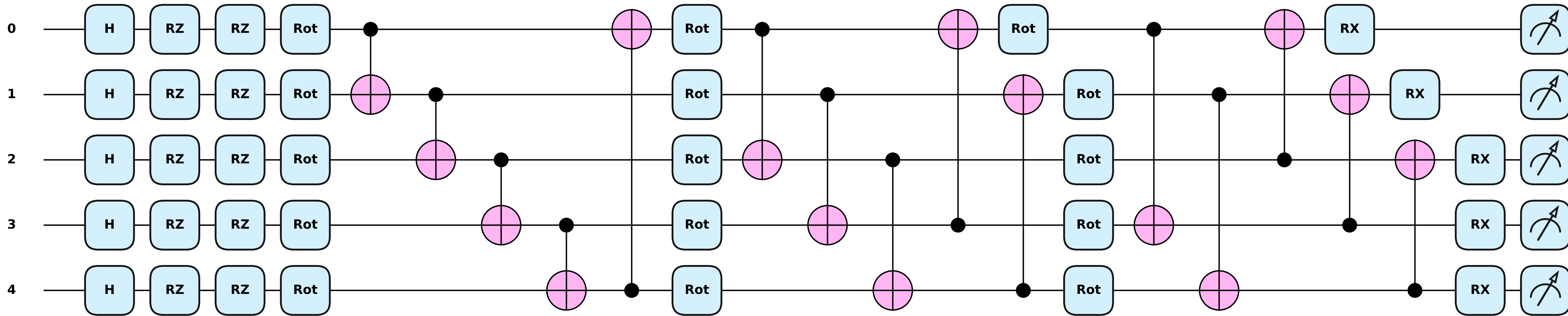
iqp_sel_55 - 5 qubits x 3 layers x range topology - 55 parameters (canonical paper circuit, frozen checkpoint epoch 1969)
