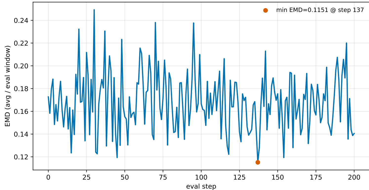
EMD over training — IQP:SEL 55p (2000ep repro)
