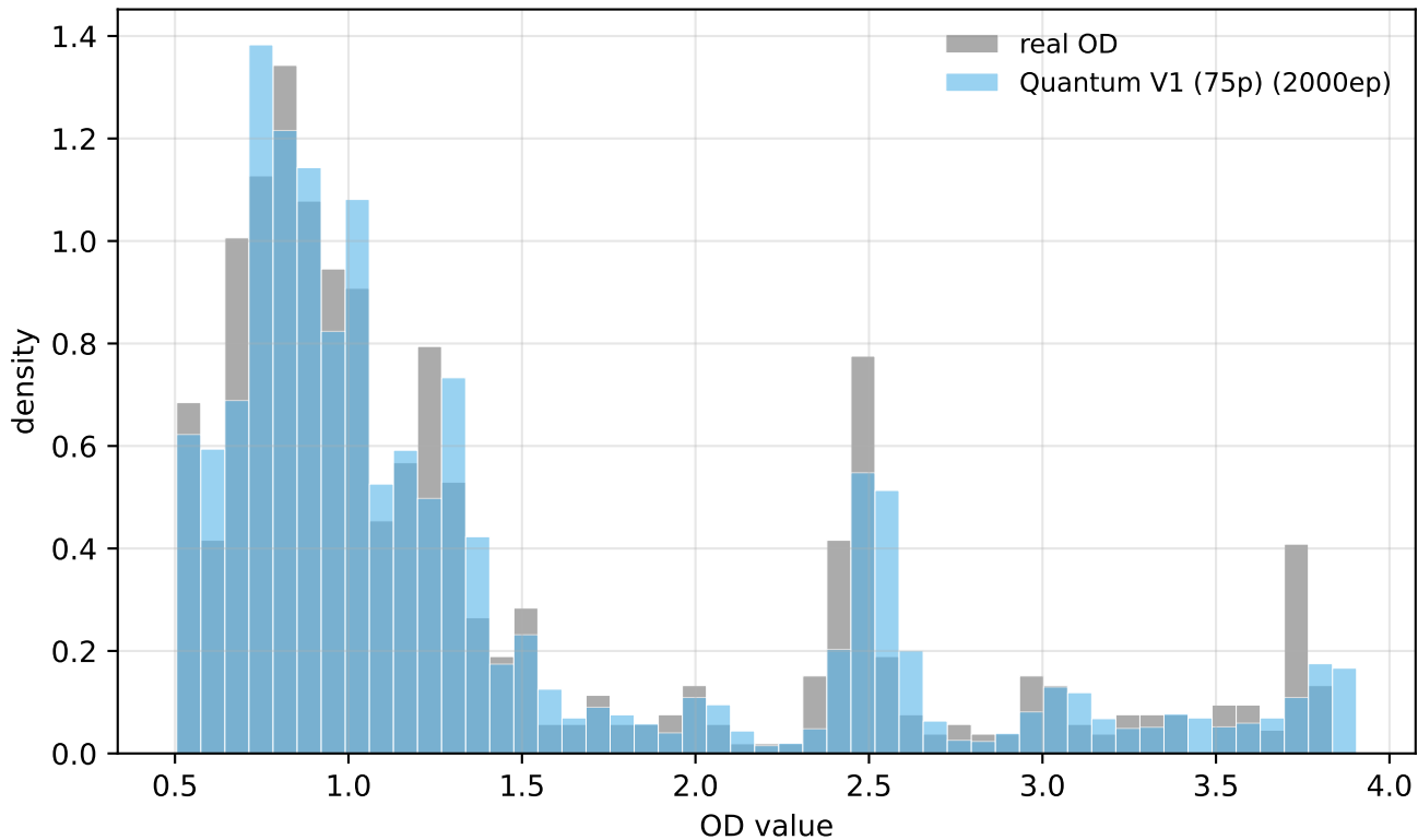
Distribution comparison — Quantum V1 (75p)
