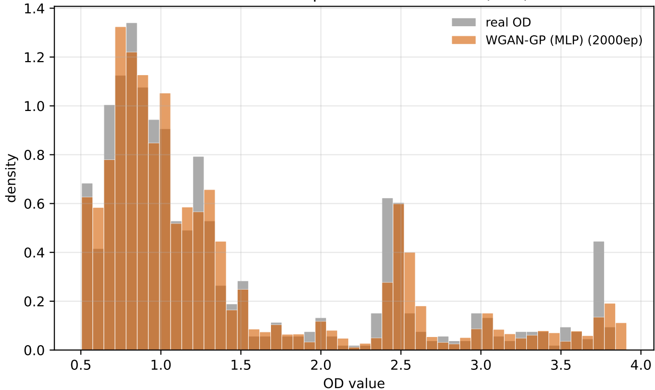
Distribution comparison — WGAN-GP (MLP)
