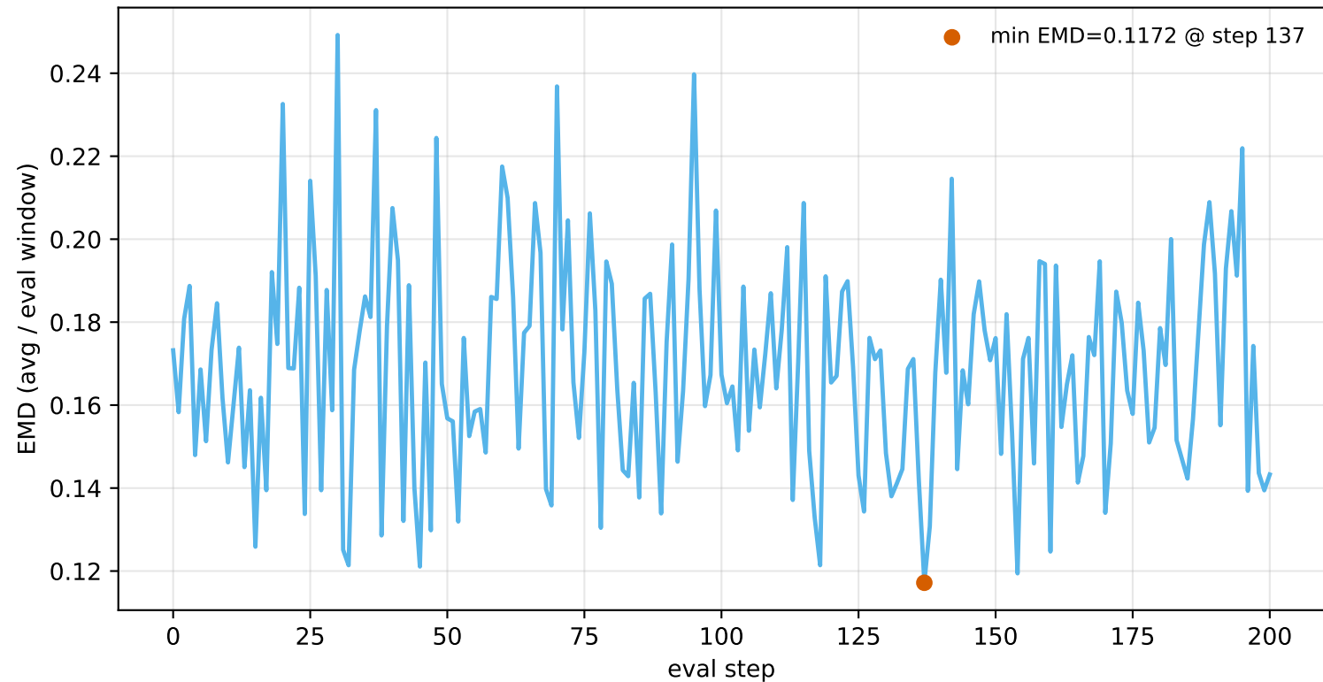
EMD over training — Quantum V1 (75p)
